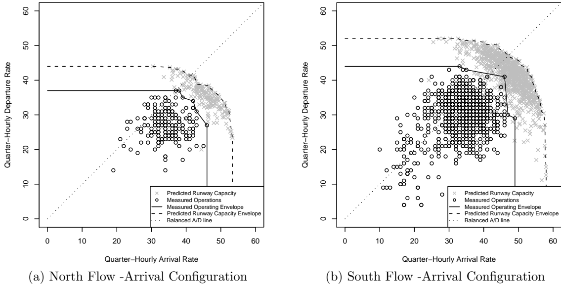
Figure 4-4: Comparison of measured airspace capacity and predicted total runway capacity for the arrival priority configurations under VMC, 5 a.m. - 12 a.m.
