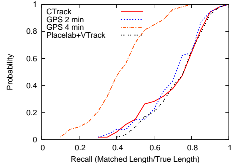
Figure 10: CDF of Recall: Comparison.
