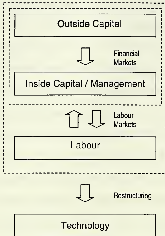
Figure 1 Specificity relations
