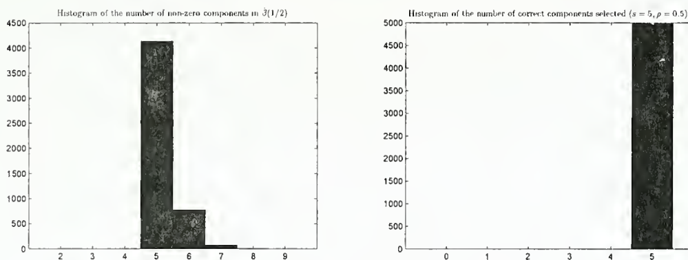
FIG 3. The figure summarizes the covariate selection results for the correlated normal design example with correlation coefficient \rho = .5 , based on 5000 Monte Carlo repetitions. The left panel plots the histogram for the number of covariates selected out of the possible 1000 covariates. The right panel plots the histogram for the number of significant covariates selected; there are in total 5 significant covariates amongst 1000 covariates. We obtained the results using 5000 Monte Carlo repetitions.
