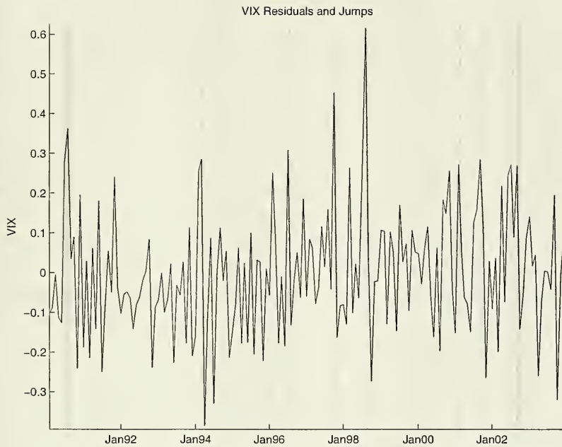
Figure 7: VIX residuals. The grey areas correspond to instances where the VIX residual is above the jump-cutoff.
