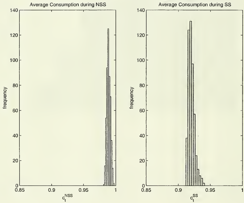
Figure 6: Average consumption during SS and NSS.
