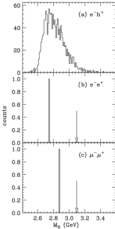
FIG. 4. Invariant mass spectra from a negative particle in the SOS and a positive particle in the HMS for events passing the timing cuts shown in Fig. 3. The arrows correspond to the J/\psi mass.
