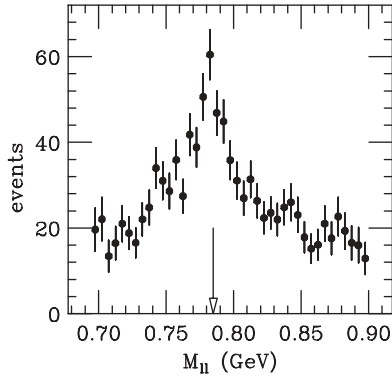
FIG. 5. Acceptance-corrected invariant mass spectrum from an electron in the SOS and a positron in the HMS, at kinematics optimized for detection of \omega(785) \rightarrow e^+e^- (indicated by the arrow) and \rho(770) \rightarrow e^+e^- .
