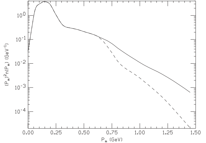
FIG. 6. The E_m -integrated probability of finding a nucleon with missing momentum P_m as a function of P_m . The solid and dashed lines are, respectively, “high” and “low” eyeball extrapolations above 0.6 GeV of the spectral function of Ref. [12].
