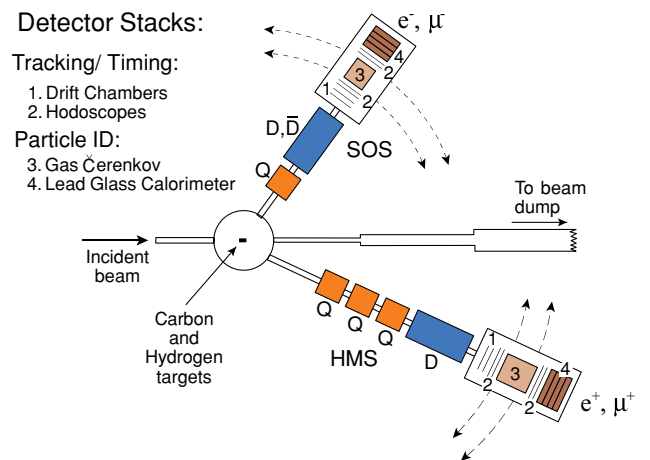
FIG. 2. (Color online) Layout of spectrometers and detectors, where Q and D represent quadrupole and dipole magnets, respectively.
