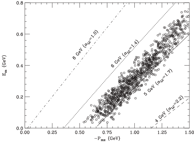
FIG. 1. The four curves show the maximum value of missing energy E_m as a function of the negative z component of missing momentum P_m , for 4-, 5-, 6-, and 8-GeV photons, for the case of quasifree photoproduction of J/\psi mesons from a nucleon bound in a nucleus. The circles represent the relative distribution of events predicted for the present experiment for the specific model described in the text (although no events were actually observed). The values of light cone fraction \alpha_{LC} are indicated for each photon energy.
