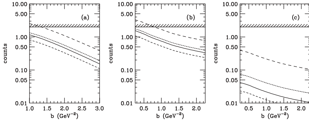
FIG. 7. The number of predicted counts for the conditions of the present experiment as a function of b for (a) model I, (b) model II, and (c) model III, where the models are defined in Eqs. (4), (5), and (6), respectively. On each panel, the solid (long dashed) curves use the “high” extrapolation of the spectral function (see Fig. 6) with (without) the E_m shift for P_m > 0.8 GeV described in the text. The medium dashed (short dashed) curves are the corresponding curves with the “low” extrapolation. The hatched band at 2 counts indicates the 87% confidence level corresponding to our experimental observation of no events.
