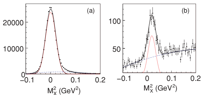
FIG. 9. (Color online) Fits to identified (a) ep\gamma and (b) ep\pi^0 final states to determine the mean values and standard deviations of the Gaussian functions G_\gamma and G_{\pi^0} . The solid line is the fit function, the dashed line is the fitted Gaussian function, and the dashed-dotted line is the polynomial fit to the radiative tail and the background.
