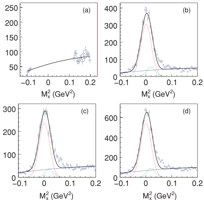
FIG. 10. (Color online) Example of fits obtained using Eq. (23) for one \phi_{p\gamma} bin. (a) Fit to the background using the end points of the M_x^2 distribution. (b), (c), and (d) are fits to the M_x^2 distributions corresponding to positive, negative, and summed beam helicity states, respectively. In (b)–(d), the fit parameters are the number of single photon and \pi^0 events; the solid lines are the fit functions as defined in Eq. (23), the dashed lines are the Gaussian functions for the single photon events, the dashed-dotted lines are the Gaussian functions for the single \pi^0 events, and the dashed-dot-dot-dot lines are the polynomial background.
