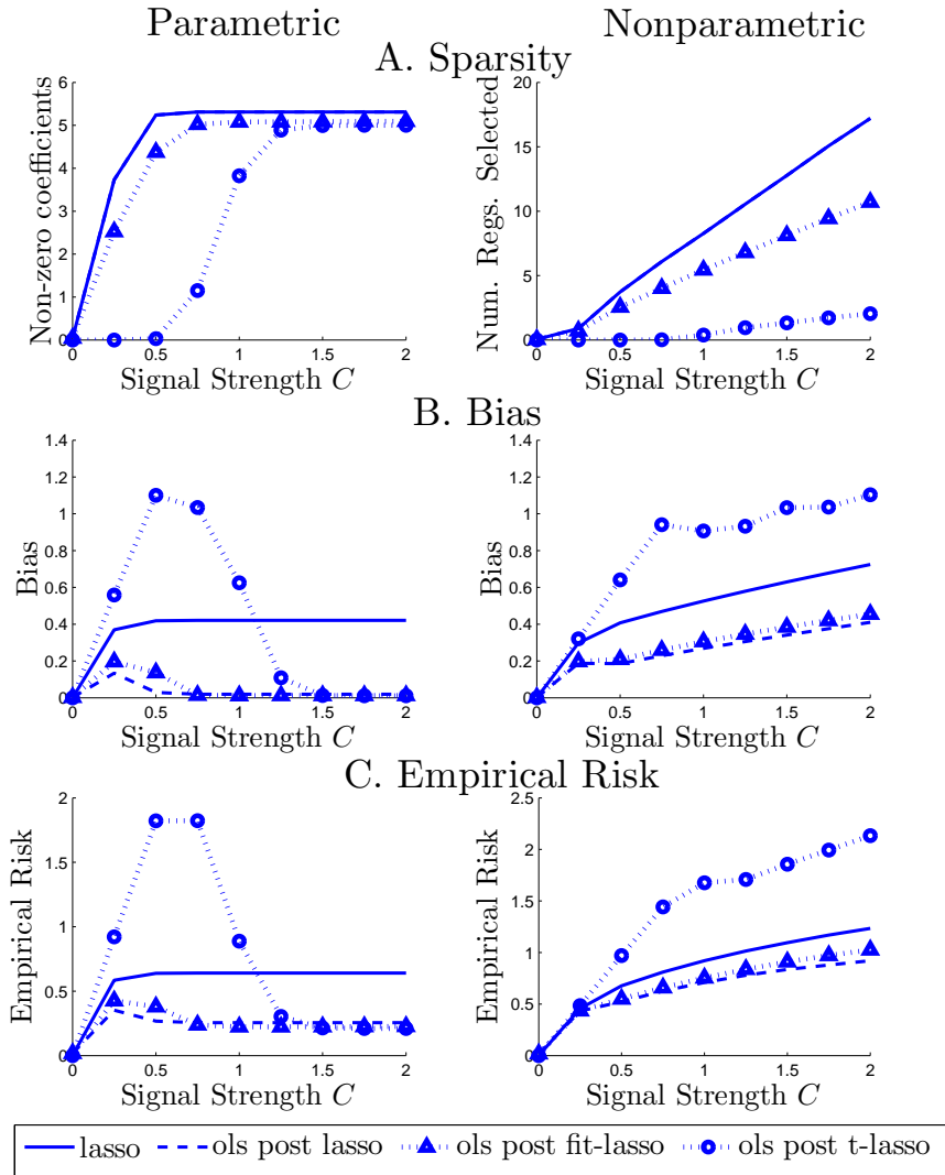
FIGURE 3. This figure plots the performance of the estimators listed in the text under the Toeplitz design for the covariates, \Sigma_{jk} = \rho^{|j-k|} if j \neq k . The left column corresponds to the parametric case and the right column corresponds to the nonparametric case described in the text. The number of regressors is p = 500 and the sample size is n = 100 with 1000 simulations for each value of C .
