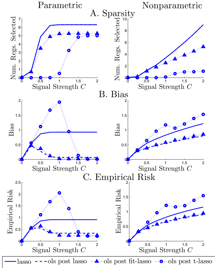
FIGURE 2. This figure plots the performance of the estimators listed in the text under the isotropic design for the covariates, \Sigma_{jk} = 0 if j \neq k . The left column corresponds to the parametric case and the right column corresponds to the nonparametric case described in the text. The number of regressors is p = 500 and the sample size is n = 100 with 1000 simulations for each value of C .
