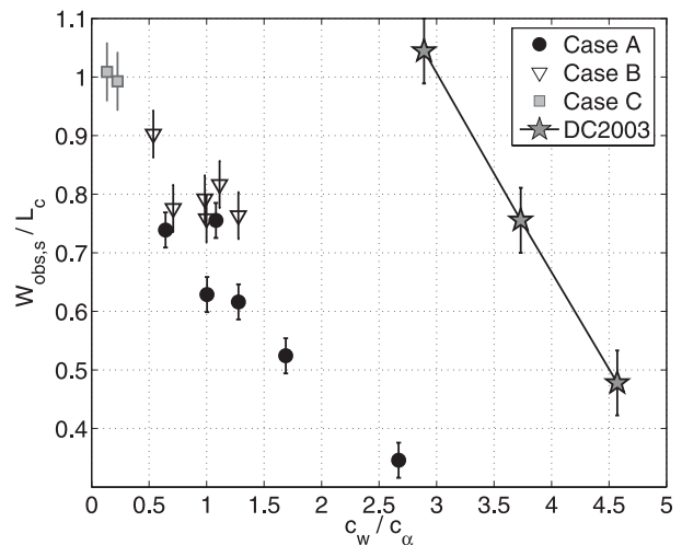
FIG. 9. Dependence of the nondimensional location of the buoyant current separation from the canyon slope, W_{obs,s}/L_c , on the degree to which bottom friction is important, indicated by c_w/c_\alpha . Stars are taken from DC03.
