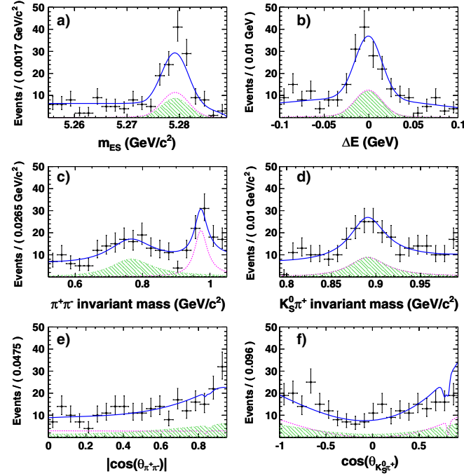
FIG. 1 (color online). Projections of the multidimensional fit onto (a) m_{ES} , (b) \Delta E , (c) \pi^+\pi^- mass, (d) K_S^0\pi^+ mass, (e) |\cos\theta_{\pi^+\pi^-}| , and (f) \cos\theta_{K_S^0\pi^+} for modes with K^{*+} \rightarrow K_S^0\pi^+ . The points with error bars show the data; the solid line shows signal-plus-background; the hatched [green] area is the \rho^0 K^{*+} signal; and the dashed [red] line is the f_0(980)K^{*+} signal.
