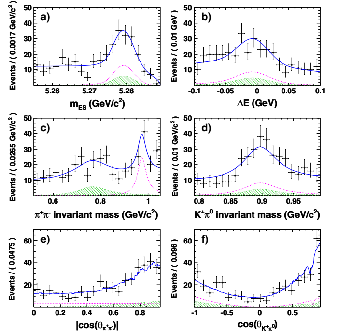
FIG. 2 (color online). Projections of the multidimensional fit onto (a) m_{ES} , (b) \Delta E , (c) \pi^+\pi^- mass, (d) K^+\pi^0 mass, (e) |\cos\theta_{\pi^+\pi^-}| , and (f) \cos\theta_{K^+\pi^0} for modes with K^{*+} \rightarrow K^+\pi^0 . The figure uses the same projection criteria and legend as Fig. 1.
