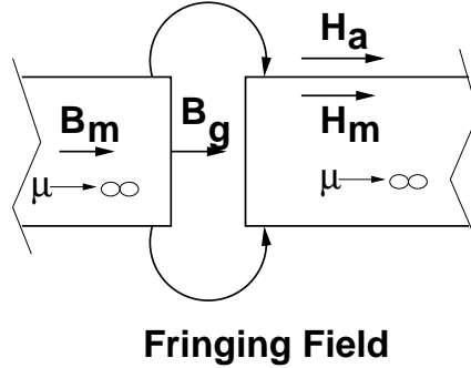
Figure 4: Gap details
