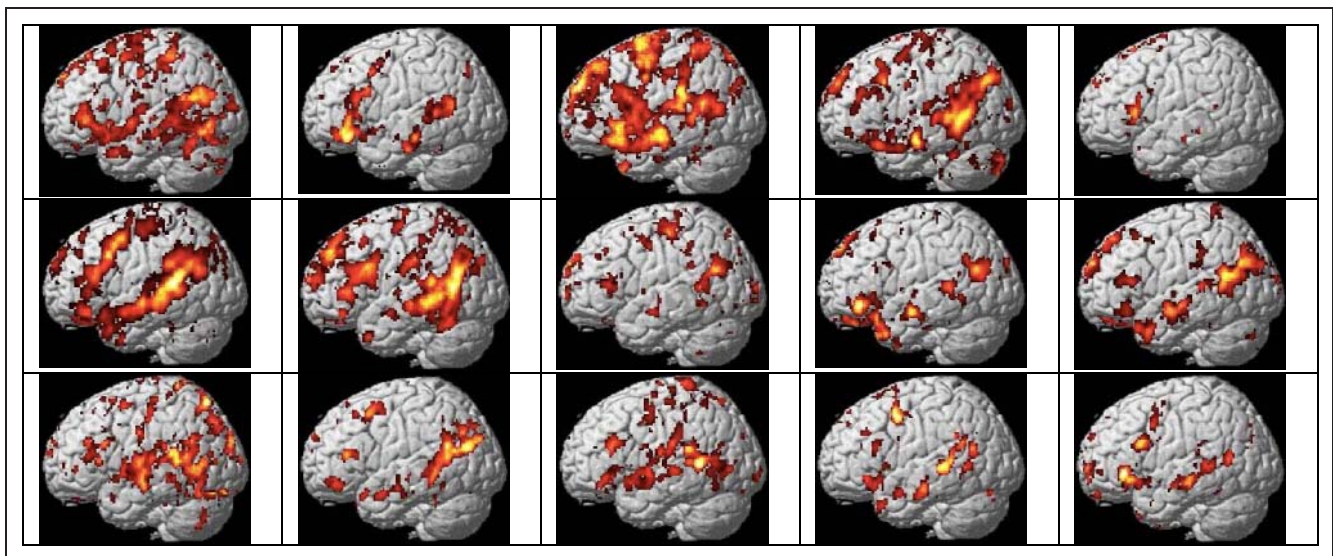
Figure 1. Sample individual activation maps from 15 subjects for the sentences > word lists contrast, thresholded at p < .001 , uncorrected. These subjects performed the version of the localizer task with a memory probe task (deciding after each sentence or word list whether a probe appeared in the immediately preceding sequence; see Fedorenko et al., 2010, for details).
