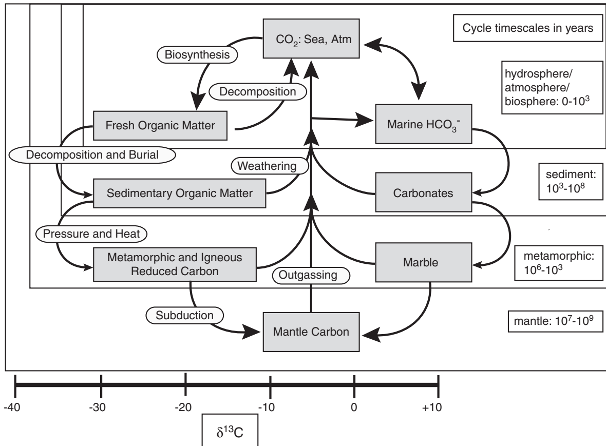
FIG. 1. Earth's biogeochemical carbon cycle, showing principal carbon reservoirs (boxes) in the mantle, crust, oceans and atmosphere, and showing the processes (arrows) that unite these reservoirs. The range of each of these reservoir boxes along the horizontal axis gives a visual estimate of typical \delta^{13}\text{C} values for each reservoir. The vertical bars at right indicate the timeframes within which C typically completely traverses each of the four subcycles. For example, carbon can traverse the hydrosphere-atmosphere-biosphere subcycle typically in the timescale between 0 and 1000 years. See Des Marais, 2001 for detailed discussion.
