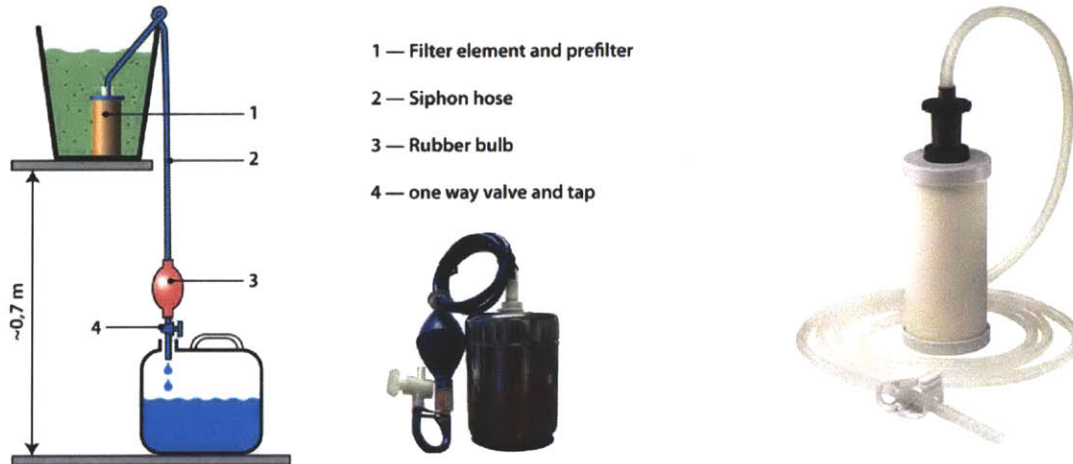
Figure 7 (a) Schematic of a Siphon Filter
