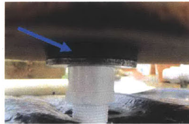
Figure 24 Rubber Connection Between Metal Washer and Ceramic Keg Source: Espinoza 2010
