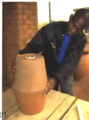
Rotating the two filters around to find the best alignment to minimize gaps between the two rims
