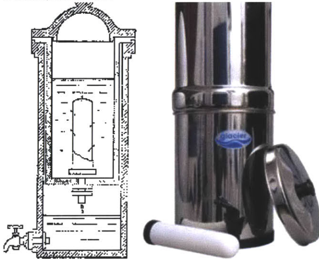
Figure 6 (left) Schematic of a Candle Filter (right) Photo of an Actual Candle Filter System Source: (left) http://www.purifiers.co.za/productinfo/121-home-units/stainless-steel-home-unit.htm (right) http://ces.iisc.ernet.in/energy/water/paper/drinkingwater/simplemethods/filtration.html
