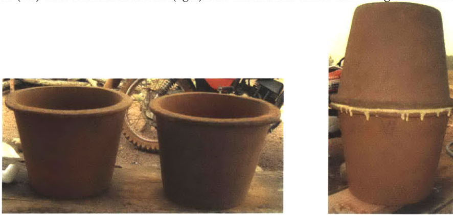
Figure 16 (left) Two Ceramic Pot Filters (right) Two Ceramic Pot Filters Sealed Together Into Keg
