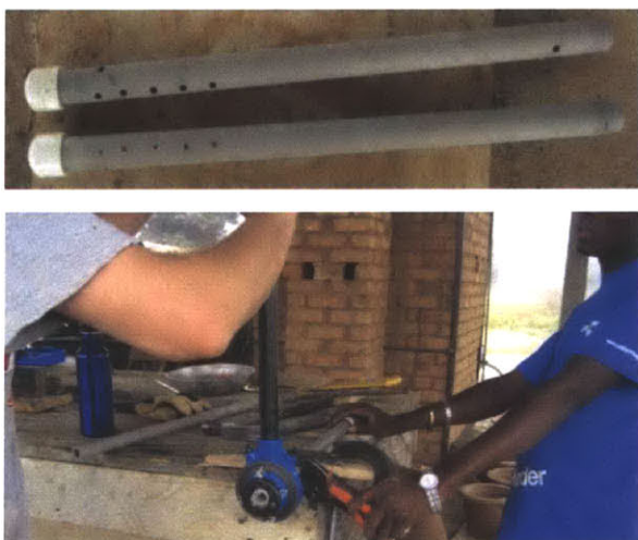
Figure 42 (top left) PVC Pipe With Holes Drilled In (bottom left) PVC Pipe Being Re-Threaded (bottom right) Screwing in PVC Riser Pipe with O-Ring Seals
