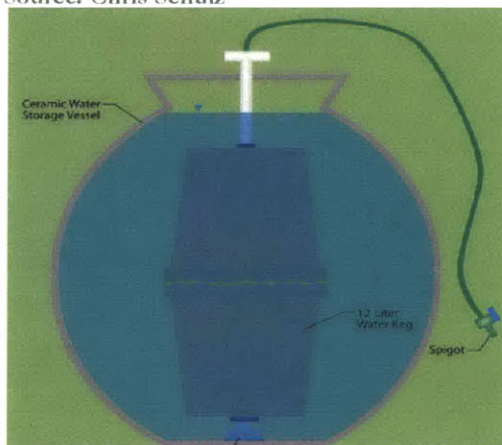
Figure 14 Schematic of Installed KWK with Siphon
