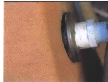
Figure 25 Ceramic Filter Breaking When Metal Washer is Attached With Epoxy Source: Espinoza 2010
