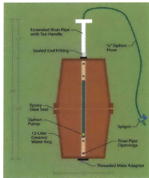
Figure 23 First Iteration KWK Source: Chris Schulz
