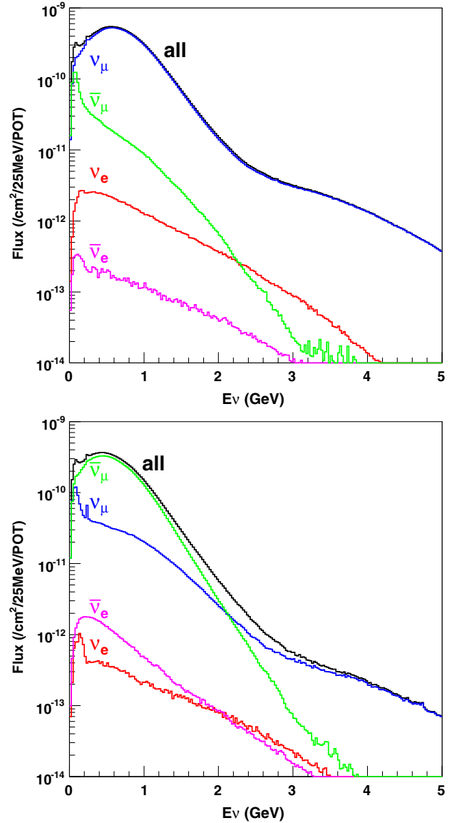
FIG. 1 (color online). Neutrino flux predictions at the SciBooNE detector as a function of neutrino energy E_\nu , normalized per unit area, POT, and neutrino energy bin width, in neutrino (top) and antineutrino (bottom) modes. The spectra is averaged within a circle with radius 2.12 m from beam center (coincides with center of detector cross-sectional area), which covers the entire 3 \text{ m} \times 3 \text{ m} cross-sectional area of the SciBooNE detector. The total flux and contributions from individual neutrino flavors are shown.
