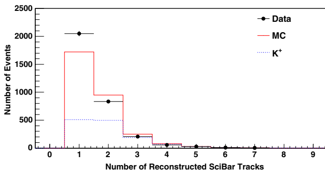
FIG. 5 (color online). Number of SciBar reconstructed tracks for the selected event sample in neutrino mode for data and NUANCE MC. MC histogram includes all events and K^+ shows the component of \nu_\mu from K^+ .
