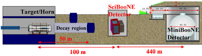
FIG. 4 (color online). Schematic overview of the Booster Neutrino Beam line and the location of the SciBooNE and the MiniBooNE detectors.
