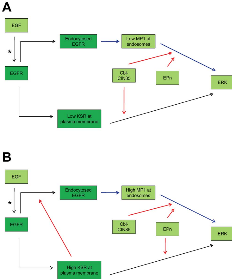
Figure 14. Distinct dynamics of EGFR endocytosis and ERK activation sensitivities mediated by scaffolds KSR and MP1, co-regulated by Cbl-CIN85 and Endophilin A1. EGF-induced ERK activation are collectively regulated at two different compartments (subpathways): near the plasma membrane (the conventional EGFR-Ras-Raf-MEK-ERK module and KSR-mediated signaling), and at late endosomes (MP1-mediated signaling). In this model, (A) when scaffold proteins are present at low levels, the two subpathways show distinctive sensitivities toward growth factor stimulation. MP1 exerts a more robust response to both endocytosed EGFR and ERK activation (lower sensitivity, denoted by blue lines) which could be influenced further by both Cbl-CIN85 and Endophilin (denoted by red lines). However, KSR has little effect on endocytosed EGFR but it affects sensitivity of ERK activation, co-regulated mainly by Cbl-CIN85 (denoted by red line) and not by Endophilin A1. (B) When both scaffold proteins are present at high levels, the sensitivity of endocytosed EGFR becomes milder and “analog-like” for the endosomal ERK activation (denoted by blue line) which is also co-regulated by both Cbl-CIN85 and Endophilin (denoted by red lines). However, high levels of KSR could now exert greater influence on the sensitivity of endocytosed EGFR (denoted by red line) to become more “digital” while the sensitivity of ERK mediated by KSR is further regulated more profoundly by Endophilin A1 (denoted by red line) but less by Cbl-CIN85. For further clarify, light green boxes denote components contributing towards lower sensitivity, high green boxes denote components contributing towards higher sensitivity. doi:10.1371/journal.pone.0022933.g014
