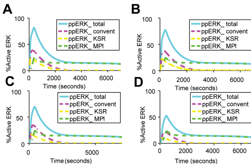
Figure 9. ERK activation regulated by membrane- and endosome-based modules. The contribution of the two membrane and one endosome components, the conventional EGFR-Ras-Raf-MEK-ERK signaling module (Convent), the KSR-mediated module (KSR), and the MP1 module (MP1), on ERK activation at various EGF concentrations: (A) 100 ng/ml, (B) 60 ng/ml, (C) 40 ng/ml, (D) 25 ng/ml. doi:10.1371/journal.pone.0022933.g009
