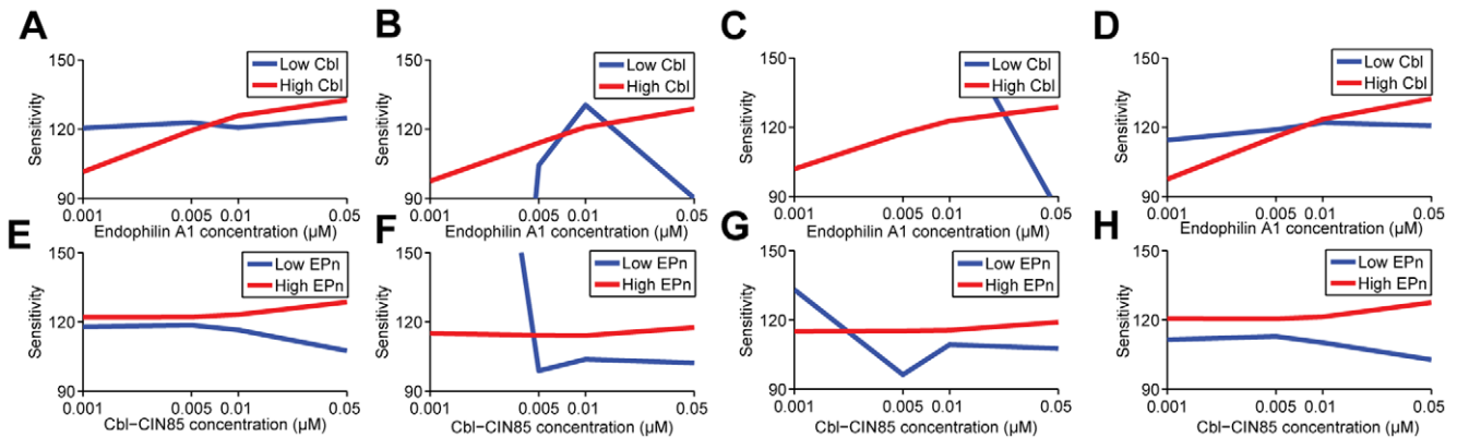
Figure 13. Detailed analysis on the sensitivities of EGFR endocytosis mediated by scaffold proteins KSR and MP1 coregulated by Cbl-CIN85 and Endophilin A1. Sensitivities of endocytosed EGFR toward EGF variation (A to D) regulated by Endophilin A1 concentration variation when Cbl-CIN85 is low (0.0001 μM) or high (0.8 μM); (E to H) Cbl-CIN85 concentration variation when Endophilin A1 is low (0.0001 μM) or high (0.8 μM) at four conditions: (A, E) when both scaffolds are present in suboptimal “low” levels [KSR = 0.02 μM, MP1 = 0.02 μM]; (B, F) when both scaffolds are present in optimally “high” concentrations as determined earlier [KSR = 0.3 μM, MP1 = 0.3 μM]; (C, G) when KSR is present at “high” level [0.3 μM] and MP1 at “low” level [0.02 μM]; (D, H) when MP1 is present at “high” level [0.3 μM] and KSR is at “low” level [0.02 μM]. doi:10.1371/journal.pone.0022933.g013
