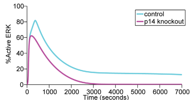
Figure 5. Profile of ERK activation before and after p14 knockout. The amount of active ERK produced in the later phase (>600 seconds) is reduced. doi:10.1371/journal.pone.0022933.g005
