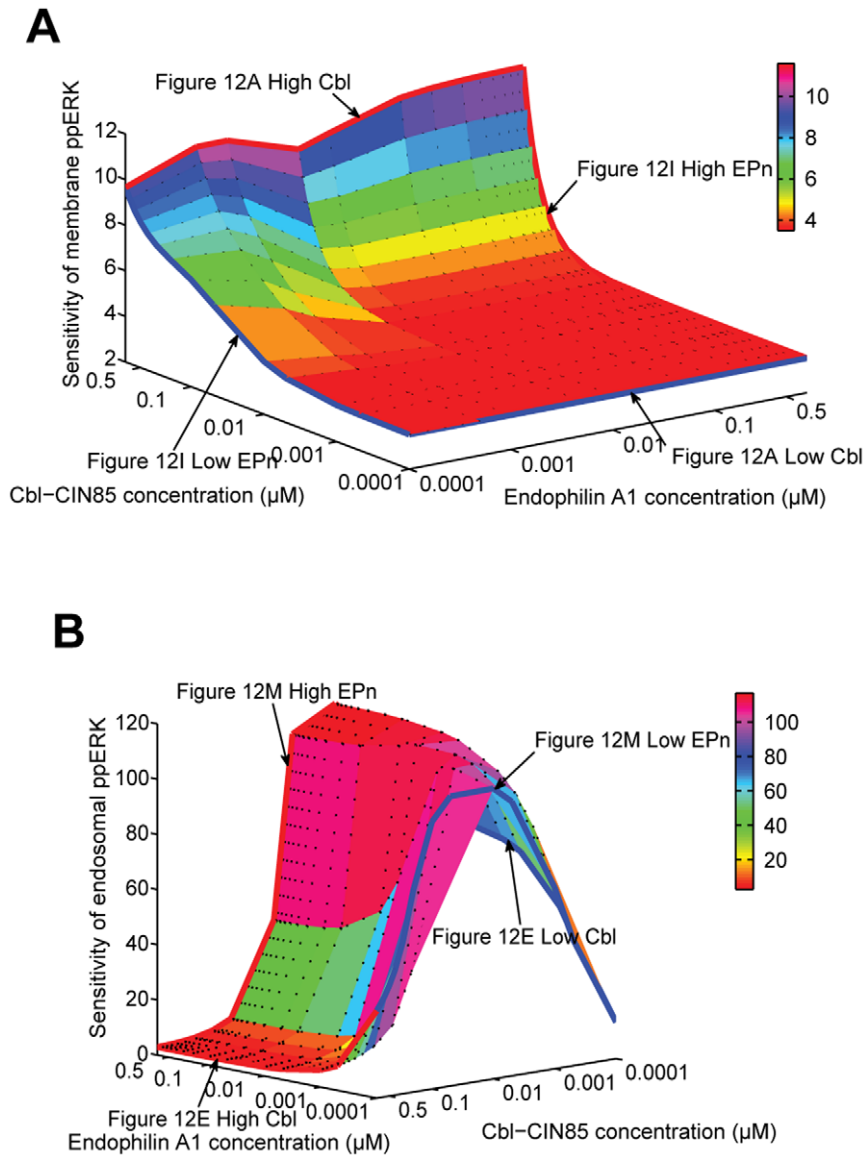
Figure 10. Differential sensitivity of ppERK from (A) membrane and (B) endosomal subpathways for EGF under various Cbl-CIN85 and Endophilin A1 concentrations when both scaffold proteins KSR and MP1 are expressed at sub-optimal “low” levels. For clarity, the sensitivity levels are denoted by colors in the scale bars. Arrows indicate response curves under the conditions specified and detailed in Figure 12, Panels A, E, I, M. doi:10.1371/journal.pone.0022933.g010
