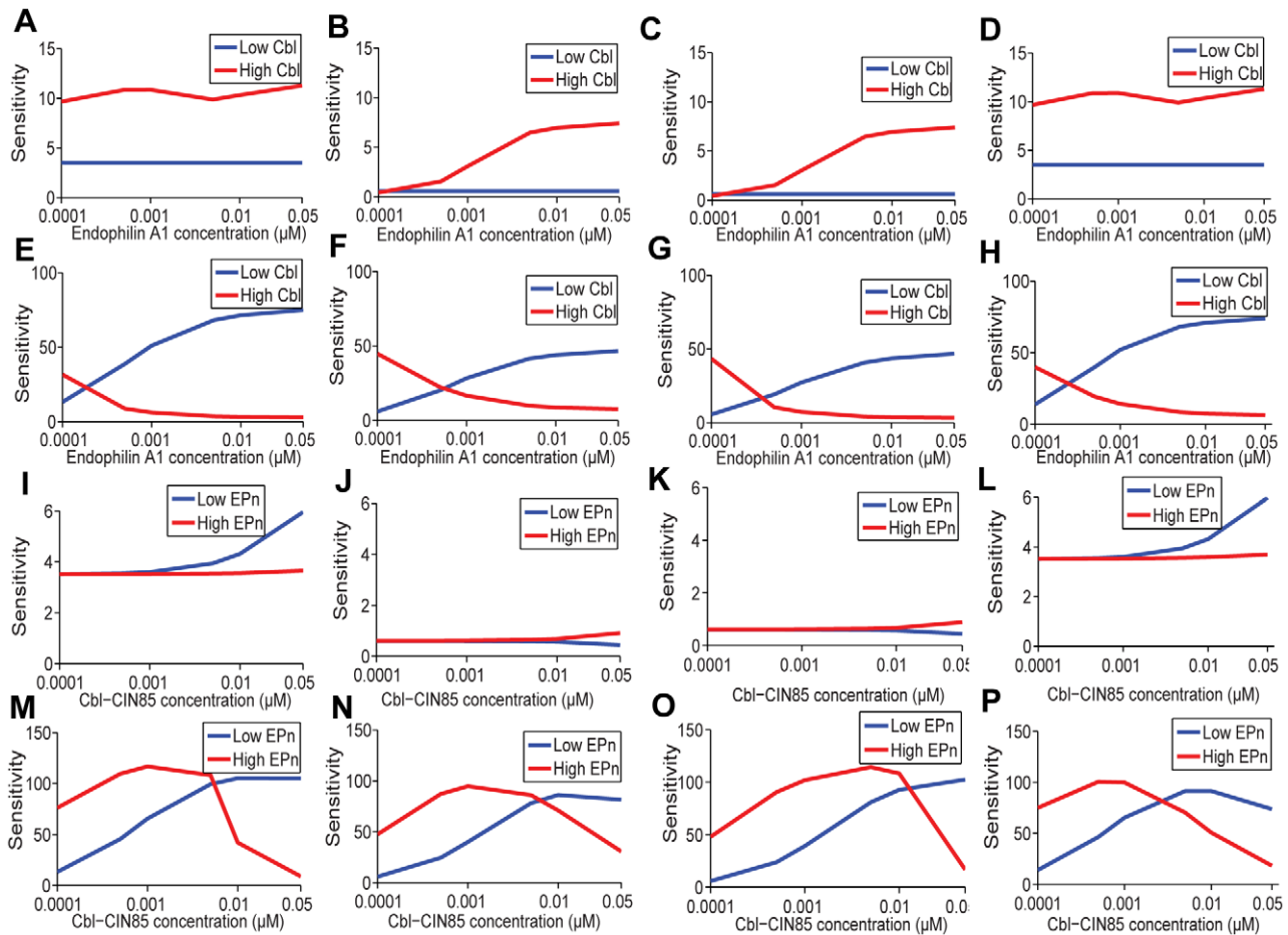
Figure 12. Detailed analysis on the sensitivities of activated ERK mediated by scaffold proteins KSR and MP1 and modulators Cbl-CIN85 and Endophilin A1 under various situations. Sensitivities of first and third panel (A, B, C, D, I, J, K, L) KSR-mediated and conventional; second and fourth panel (E, F, G, H, M, N, O, P) MP1-mediated subpathways toward EGF variation regulated by (A - H) Endophilin A1 concentration variation when Cbl-CIN85 is low (0.0001 μM) or high (0.8 μM); (I - P) Cbl-CIN85 concentration variation when Endophilin A1 is low or high at four conditions: (A, E, I, M) when both scaffolds are present in suboptimal “low” levels [KSR = 0.02 μM, MP1 = 0.02 μM]; (B, F, J, N) when both scaffolds are present in optimally “high” concentrations as determined earlier [KSR = 0.3 μM, MP1 = 0.3 μM]; (C, G, K, O) when KSR is present at “high” level [0.3 μM] and MP1 at “low” level [0.02 μM]; (D, H, L, P) when MP1 is present at “high” level [0.3 μM] and KSR is at “low” level [0.02 μM]. doi:10.1371/journal.pone.0022933.g012
