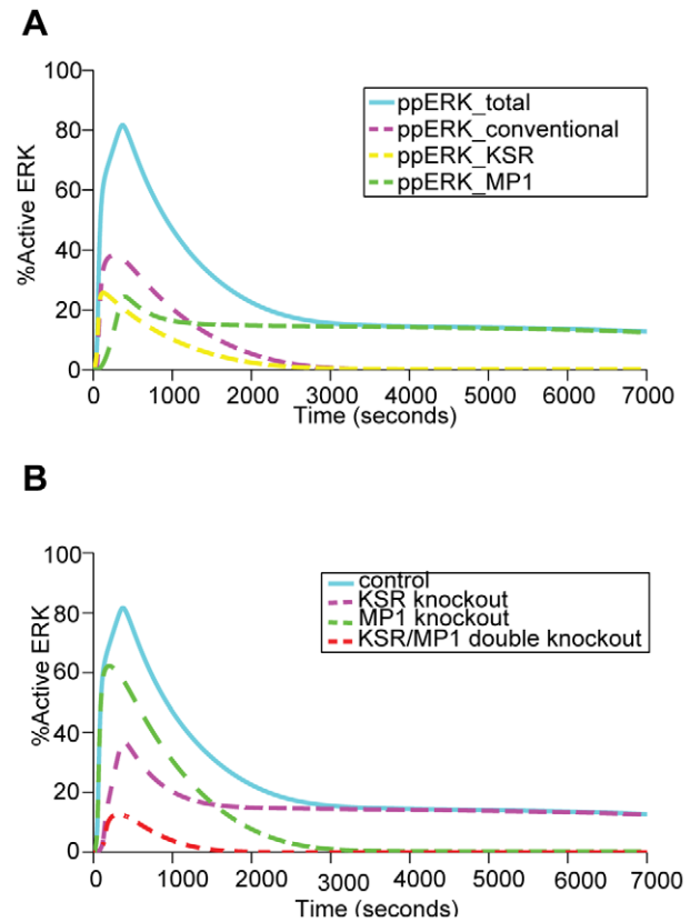
Figure 7. The collective effect of scaffold proteins KSR and MP1 on ERK activation. (A) Overall signaling and contribution from individual modules. (B) Signaling profile under knockout conditions. doi:10.1371/journal.pone.0022933.g007
