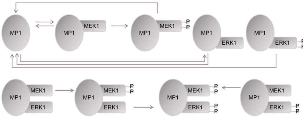
Figure 3. A detailed biochemical model of scaffolding action of MP1. Please refer to “Methods” for the considerations and assumptions used and Supplementary Table S1 for detailed descriptions of their kinetics parameters. “P” denotes protein phosphorylation. doi:10.1371/journal.pone.0022933.g003
