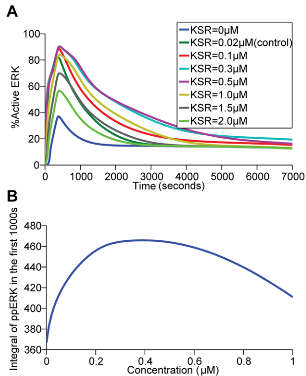
Figure 4. The biphasic effect of KSR on ERK activation. (A) Percentage of active ERK was plotted over the period indicated by varying the concentrations of KSR from 0 to 2 \mu M. (B) Existence of an optimal scaffold concentration of KSR (0.3–0.5 \mu M) by plotting the time integral of ppERK/ERK in the first 1000 seconds and KSR’s initial concentrations. doi:10.1371/journal.pone.0022933.g004
