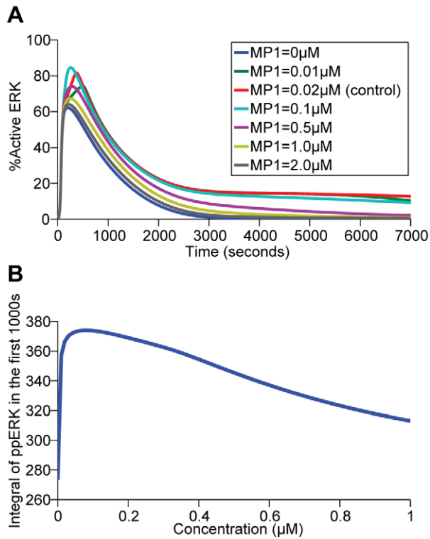
Figure 6. The biphasic effect of MP1 on ERK activation. (A) Percentage of active ERK was plotted over the period indicated by varying the concentrations of MP1 from 0 to 2 \mu\text{M} . (B) Existence of an optimal scaffold concentration of MP1 (0.1 \mu\text{M} ) by plotting the time integral of ppERK/ERK in the first 1000 seconds and MP1's initial concentrations. doi:10.1371/journal.pone.0022933.g006
