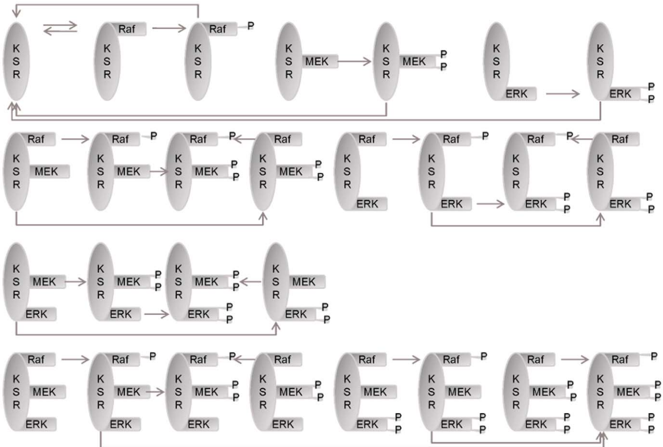
Figure 2. A detailed biochemical model of scaffolding action of KSR. Please refer to “Methods” for the considerations and assumptions used and Supplementary Table S1 for detailed descriptions of the kinetics parameters. “P” denotes protein phosphorylation. doi:10.1371/journal.pone.0022933.g002
