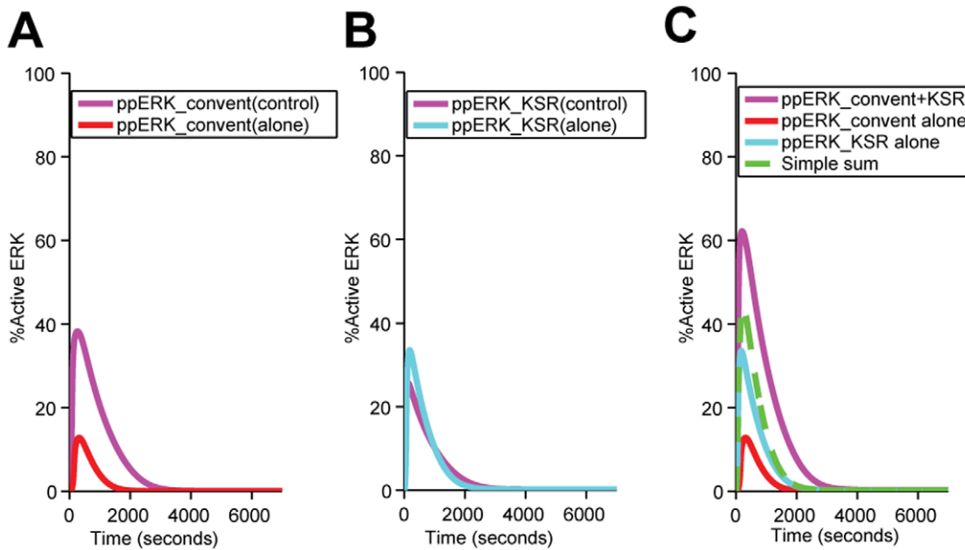
Figure 8. The synergistic effect of the two membrane associated signaling components, the conventional EGFR-Ras-Raf-MEK-ERK signaling module (Convent) and the KSR-mediated module (KSR) on ERK activation. doi:10.1371/journal.pone.0022933.g008
