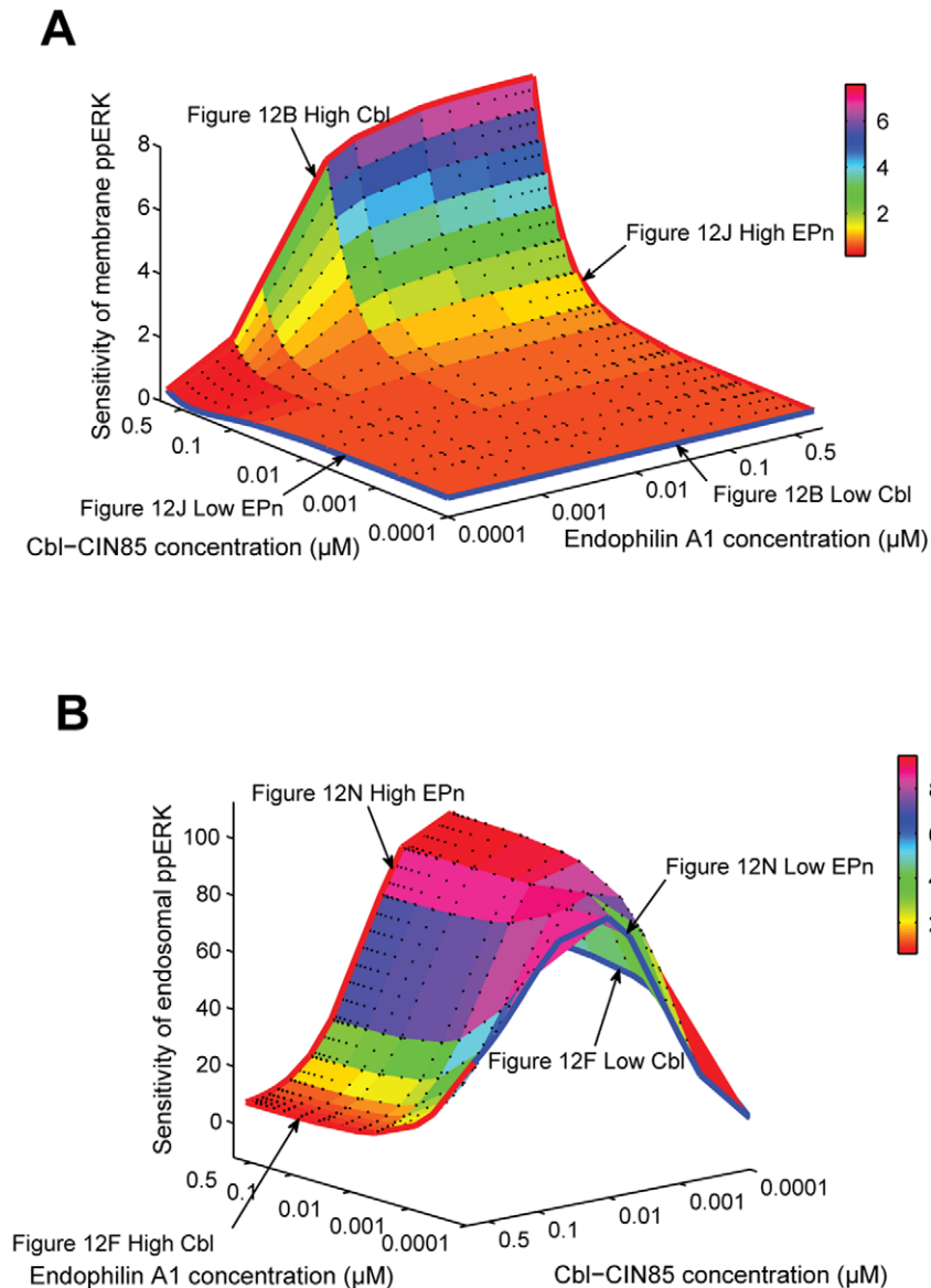
Figure 11. Differential sensitivity of ppERK from (A) membrane and (B) endosomal subpathways for EGF under various Cbl-CIN85 and Endophilin A1 concentrations when scaffold proteins KSR and MP1 are highly expressed – optimal for signaling. For clarity, the sensitivity levels are denoted by colors in the scale bars. Arrows indicate response curves under the conditions specified and detailed in Figure 12, Panels B, F, J, N.
