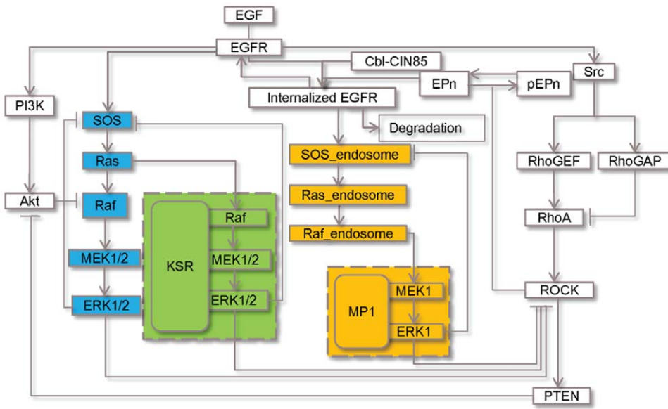
Figure 1. A model for Ras/ERK signaling pathway regulated by scaffolds and modulators. More detailed biochemical model of scaffolding actions of KSR and MP1 in the dashed rectangular boxes are shown in Figures 2 and 3, respectively. Molecules highlighted in blue, green and orange boxes represent the separate modules of Ras/ERK signaling operating from the conventional mode (no-scaffolds; membrane), KSR-supported mode (membrane) and MP1-supported mode (late endosome), respectively. doi:10.1371/journal.pone.0022933.g001
