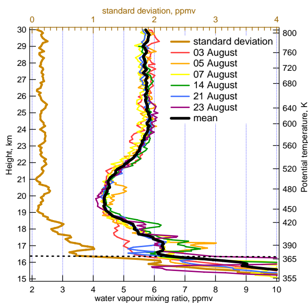
Fig. 2. Individual and mean water vapour profiles of the six soundings (bottom axis) and standard deviation (brown, top axis). The mean tropopause level is shown by black dashed line.
