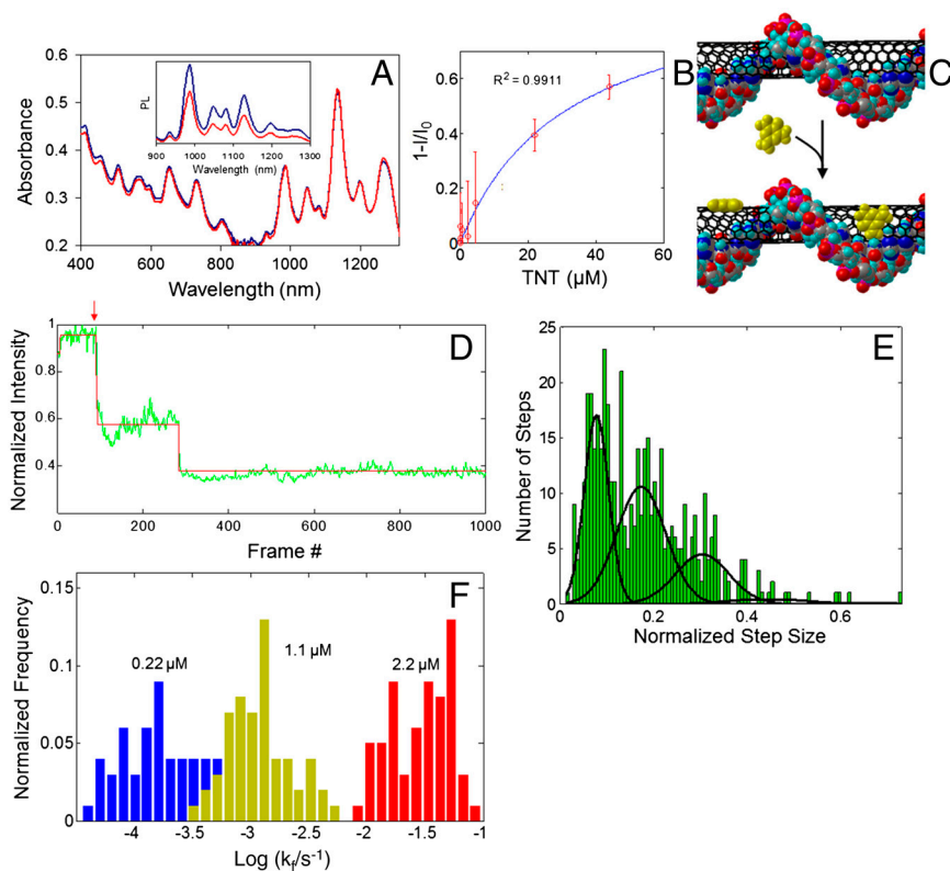
Fig. 6. Single-molecule, reversible excitonic quenching of ss(AT) 15 -SWNT by TNT. (A) Absorption spectra of ss(AT) 15 -SWNT before (blue) and after (red) introduction of 44 μM TNT. (Inset) PL spectra under same conditions. (B) Langmuir adsorption isotherm of TNT binding to the ss(AT) 15 -encapsulated (8,7) SWNT species. (C) Depiction of direct TNT binding to the SWNT surface of the ss(AT) 15 -SWNT complex. (D) Single-molecule TNT detection by ss(AT) 15 -SWNT complexes bound to glass. The trace shows the PL of a single complex acquired under 658-nm excitation. TNT (220 nM) was added at frame 100 (red arrow); one frame was acquired every 500 ms. Intensity fluctuations were fit by an error-minimizing algorithm (red). (E) A histogram of fitted intensity fluctuations from multiple nanotube intensity traces upon exposure of SWNT to 1.1 μM TNT. The histogram, fit by a series of Gaussian curves, elucidates quantization into single, double, and triple steps. (F) Histogram of quenching rates of individual nanotubes exposed to three different concentrations of TNT.
