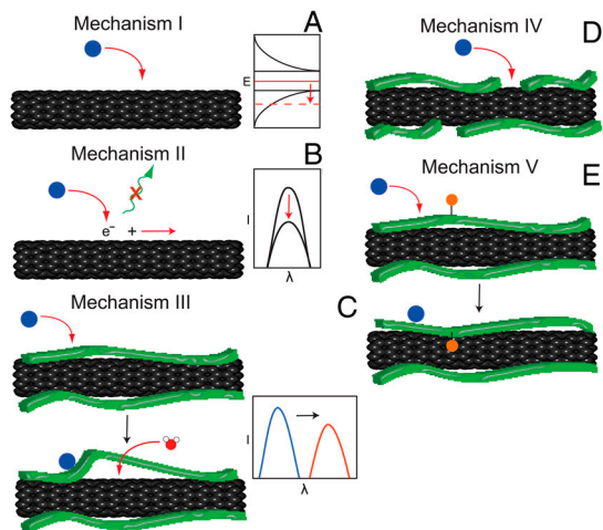
Fig. 1. Mechanisms of SWNT PL modulation. (A) Mechanism I, Fermi level shifting via redox-active analyte adsorption to the nanotube surface. (B) Mechanism II, quenching induced by exciton disruption in response to analyte binding. (C) Mechanism III, solvatochromic shifting due to perturbation of a SWNT-bound polymer. (D) Mechanism IV, selectivity of analyte binding mediated by polymer wrapping. (E) Mechanism V, analyte-activated polymer switching resulting in intensity and/or wavelength modulation.
