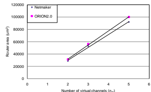
Fig. 12: Router area vs. number of virtual channels.
