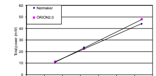
Fig. 7: Router total power vs. flit width.
