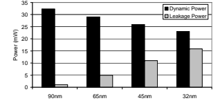
Fig. 3: Router power vs. tech. node with NVT transistors.
