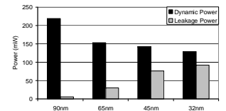
Fig. 5: Router power vs. tech. node with LVT transistors.
