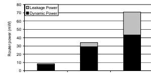
Fig. 2: Power consumption vs. transistor type.
