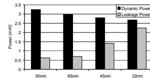
Fig. 4: Router power vs. tech. node with HVT transistors.
