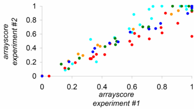
Figure S3. Reproducibility of the array experiments. Five solution probes measured in separate experiments are shown as a scatter plot. Arrayscore values >1 are set to 1. Blue, SYNZIP5 ( R^2=.99 ). Orange, SYNZIP6 ( R^2=.99 ). Teal, SYNZIP37 ( R^2=.91 ). Red, FOS ( R^2=.95 ). Green, ATF4 ( R^2=.99 ).
