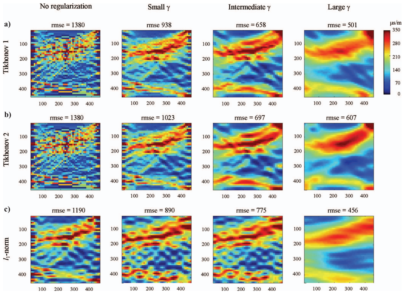
Figure 9. Cross-well traveltime tomography of the model shown in Figure 7b after adding 10% noise to data. Reconstruction results for Tikhonov regularization with (a) first-order and (b) second-order spatial derivative minimization, and (c) l_1 -norm regularization (LMN) in the DCT domain are shown with increasing regularization weight \gamma (from left to right). The root mean squared error (rmse) is in ( \mu\text{s}/\text{m} ) unit.
