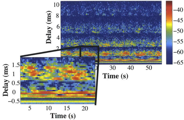
Figure 3.1.1: The magnitude of an estimated channel impulse response at 1 km from the transmitter (SPACE08 experiment).
