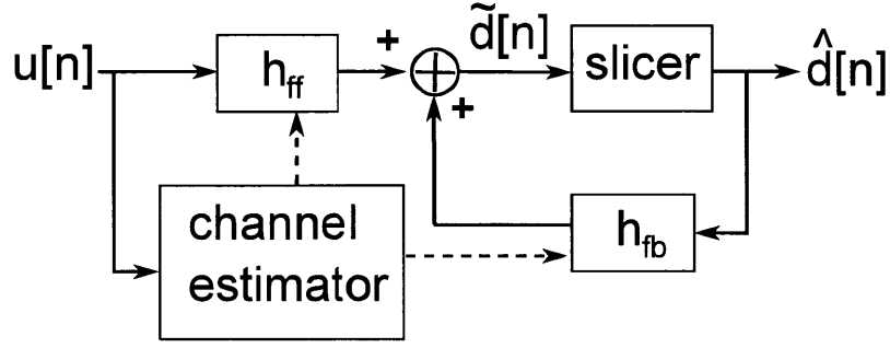
Figure 3.2.1: Illustration of the structure of a CEB-DFE.
