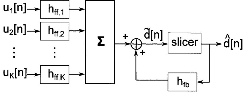
Figure 4.2.1: A multichannel decision feedback equalizer.
