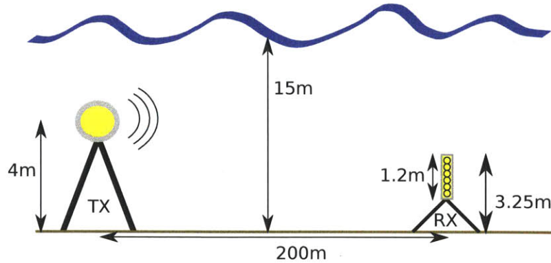
Figure 4.7.1: Setup of SPACE08 experiment
