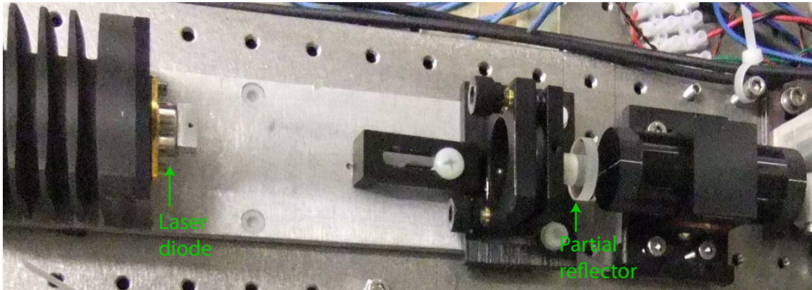
Figure A-5: Simple setup for narrowing a DFB laser by optical feedback, as described in the text.
