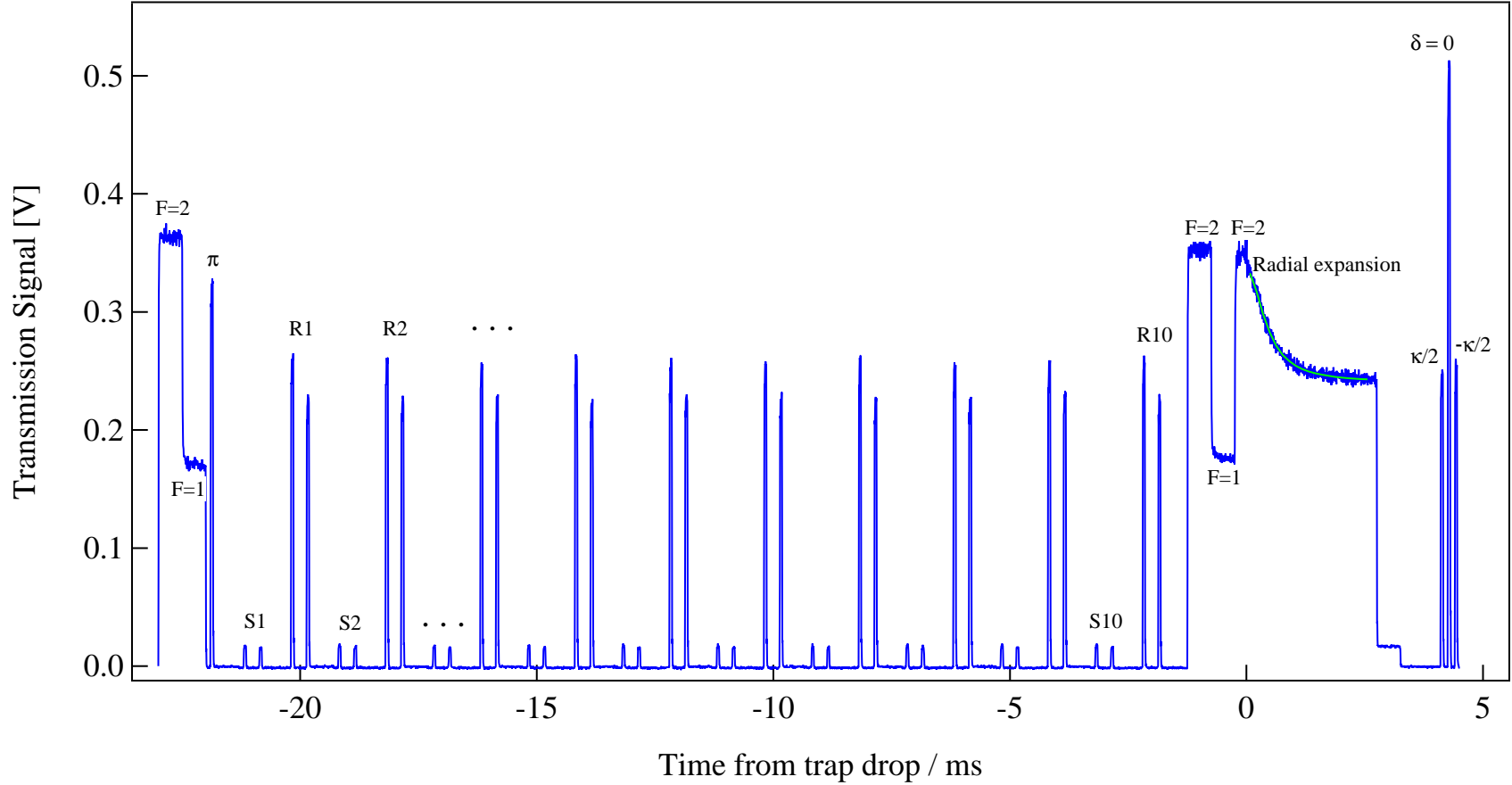
Figure 4-1: Typical trace of cavity transmission vs. time, obtained with the single-sideband probing scheme described in Sec. 3.4. Atoms are optically pumped into F=2 and F=1 to measure atom number. The light is briefly turned off to apply a \pi pulse, then pulsed back on to measure the resulting population transfer, which reflects both the optical pumping purity and the fidelity of the simple \pi pulse. Next, ten iterations of cavity feedback squeezing at low probe intensity (S1...S10) and readout at high probe intensity (R1...R10) are performed. Afterwards, the atom number is measured again. Releasing the atoms from the trap and fitting the transmission measured during the radial expansion allows for determination of the radial temperature. Finally, the probe-cavity detuning \delta \approx \kappa/2 is verified by changing it in two steps of -\kappa/2 and comparing the observed transmission to the known Lorentzian lineshape.
