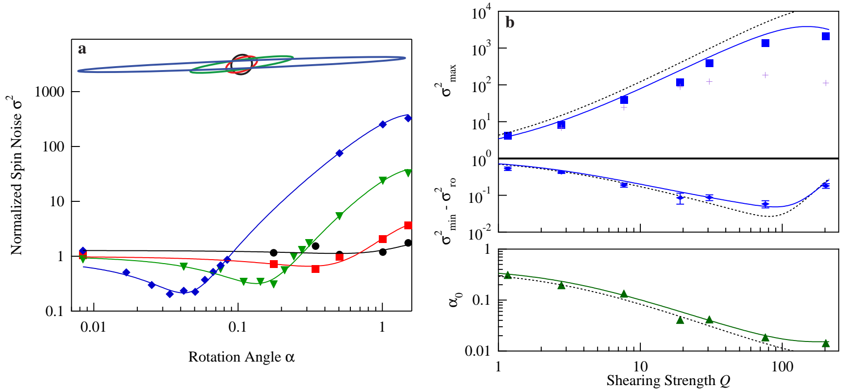
Figure 6-4: Geometry of the squeezed states prepared by cavity feedback, as determined by rotating each state by a variable angle \alpha about the mean spin \langle \mathbf{S} \rangle between squeezing and readout of S_z . The normalized spin variance \sigma^2(\alpha) = 2\Delta S_z^2/S thus measured is shown in the left graph for shearing parameters Q = 0 (black), 1.2 (red), 7.7 (green) and 31 (blue); the ellipses in the inset are polar plots of \sigma(\alpha) as given by the sinusoidal fits to the data. The maximum spin variance \sigma_{\max}^2 , minimum spin variance \sigma_{\min}^2 - \sigma_{\text{ro}}^2 with readout noise subtracted, and angle \alpha_0 of the minor axis from \hat{z} are summarized in the right graph and compared to both the idealized theory in Sec. 6.1 (black dotted curves) and a model accounting for contrast reduction and technical light noise (solid curves). The purple crosses show the maximum spin variance conditioned on the information in the detected squeezing light, as discussed in Sec. 6.4.
