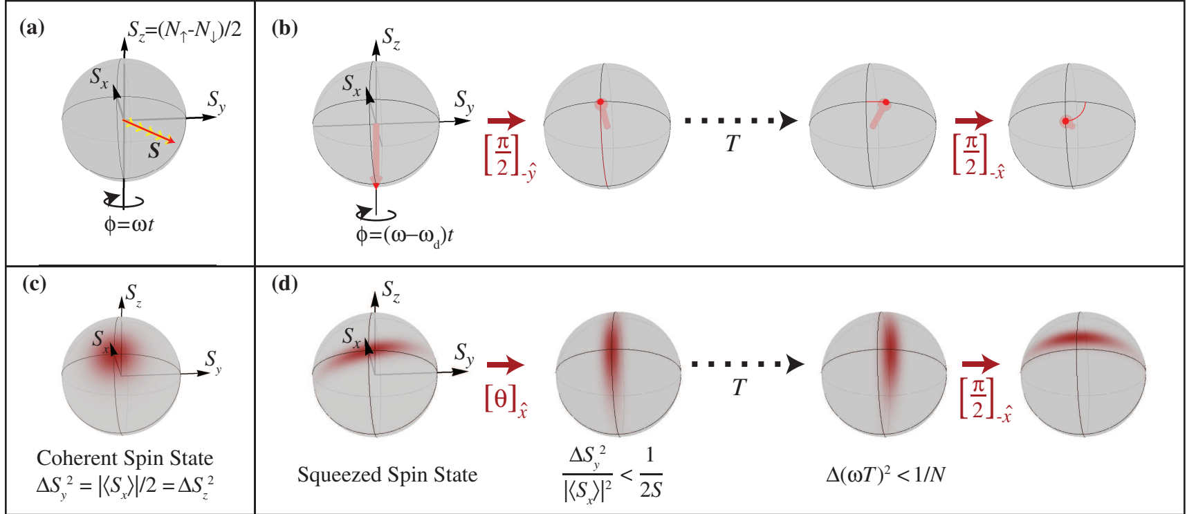
Figure 1-2: (a) Bloch-sphere representation of an ensemble of N two-level atoms as a spin vector \mathbf{S} = \sum_{i=1}^N \mathbf{s}_i (red) formed by summing the single-atom spins \mathbf{s}_i (yellow). The azimuthal angle \phi represents the phase \phi = \omega t of the spin precession, where the precession rate is set by the energy difference \hbar\omega between states |\uparrow\rangle and |\downarrow\rangle . The spin component S_z is directly proportional to the difference in populations N_\uparrow, N_\downarrow of the two spin states. (b) Ramsey sequence for measurement of the clock transition frequency \omega , illustrated in a rotating frame at the drive frequency \omega_d , as described in text. Each arrow labeled [\frac{\pi}{2}]_{\hat{r}} indicates a \pi/2 rotation about the axis \hat{r} . (c) Schematic illustration of a coherent spin state along \hat{x} on the Bloch sphere; the red shading represents a tomographic probability distribution [31] for spin components in the yz plane, with variances \Delta S_y^2 = |\langle S_x \rangle|/2 = \Delta S_z^2 set by the length |\langle S_x \rangle| = S of the ensemble spin vector for the totally symmetric state. (d) Modified Ramsey sequence incorporating a squeezed spin state. The sequence is initiated by placing the state into the phase-squeezed orientation, so that the reduced quantum uncertainty \Delta\phi^2 = \Delta S_y^2/|\langle S_x \rangle|^2 < 1/(2S) will allow the phase \phi = \omega T acquired in the precession time T to be determined to better than the standard quantum limit.
