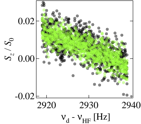
Figure 7-2: A small portion of a Ramsey fringe obtained with either a CSS (black) or a squeezed state (green). The abscissa \nu_d - \nu_{\text{HF}} represents the detuning of the microwave oscillator from the free-space |F = 1, m_F = 0\rangle \rightarrow |F = 2, m_F = 0\rangle transition. In this particular data set, the squeezed state outperforms the unentangled state by 3.2 dB in signal-to-noise ratio.
