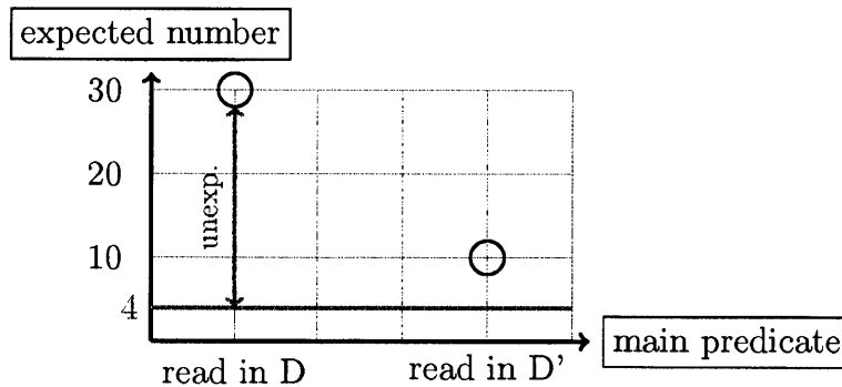
Figure 2-9: Expected number of people reading that dissertation sometime in x . Indication of the unexpectedness of exactly four people reading that dissertation in D .
