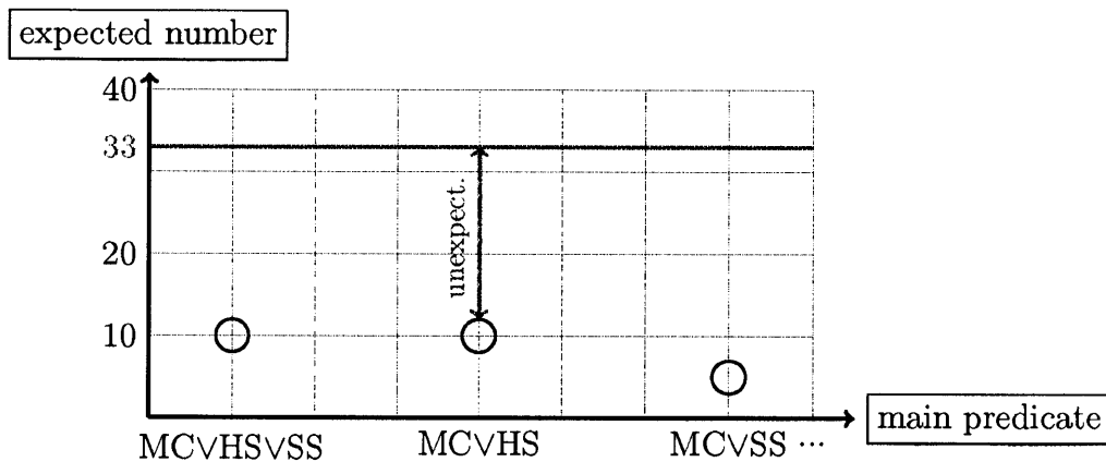
Figure 2-10: Expected number of senators reading a book by Chomsky in x . Indication of the unexpectedness of exactly thirty-three senators reading MCVHS.
