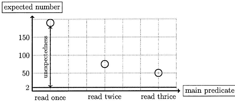
Figure 2-4: Expected number of congressmen reading the constitution x times. Indication of the unexpectedness of exactly two congressmen reading the constitution once.
