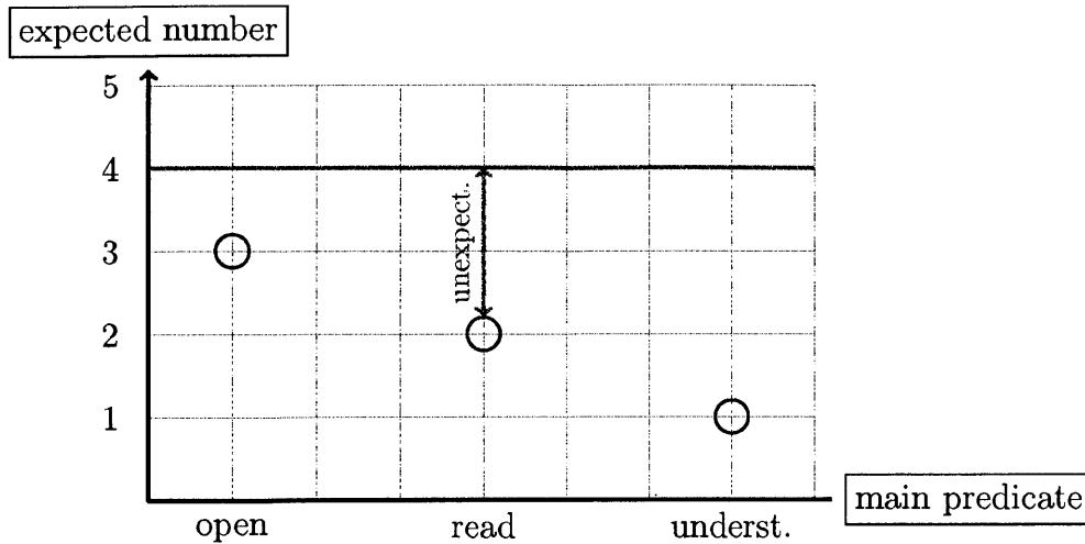
Figure 2-5: Expected number of people attending having x that dissertation. Indication of the unexpectedness of exactly four people attending the seminar having read that dissertation.
