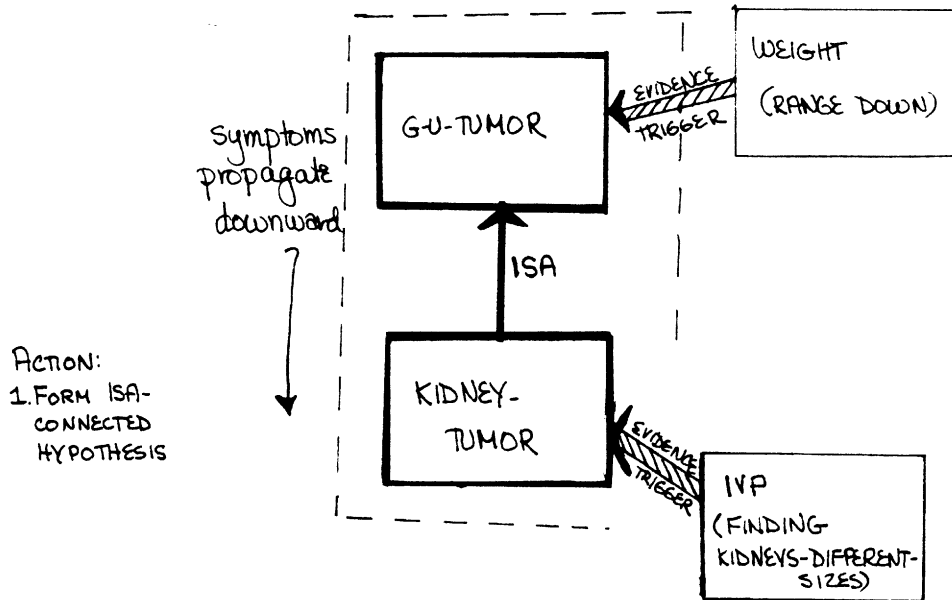
Diagram 6-4: ISA-CONNECTED TEMPLATE
