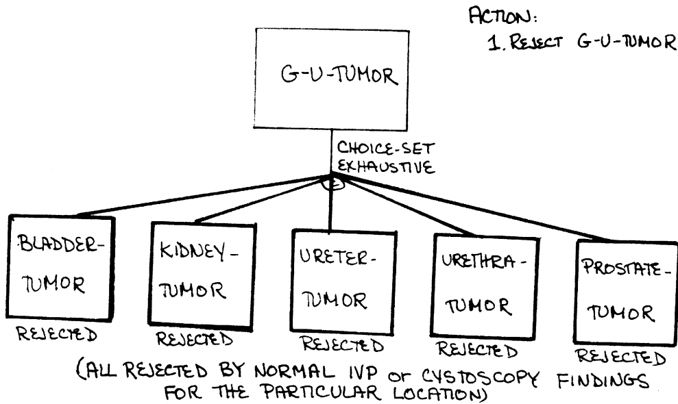
Diagram 6-17: CHOICE-SET REJECTION
