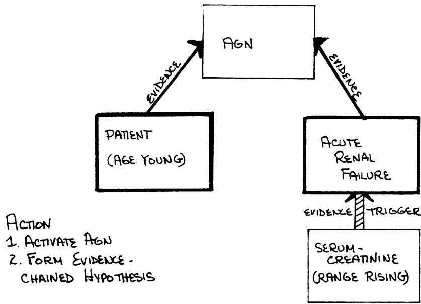
Diagram 6-8: EVIDENCE-CHAINED TEMPLATE
