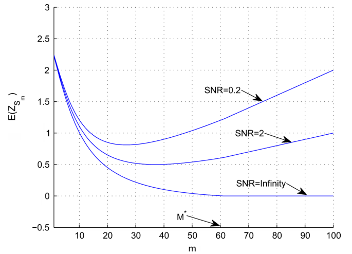
Fig. 2. Typical behavior of the expected value of the reconstruction error as the SNR (the noise variance) changes when the true parameter's order is M^* = 60 and the maximum subspace order is M = 100 (fixed data length, fixed signal power).
