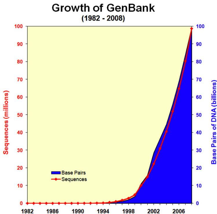
Figure 1. Growth of the publicly available gene-sequence database from its inception through 2008. 30 As of mid-2009 the number of sequences had reached 106,073,709 containing 105,277,306,080 bases. 31 Note that for the purpose of this illustration, a “base pair” is synonymous with a base.
