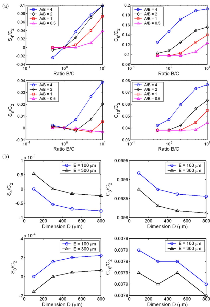
Fig. 3. (a) Coefficients for the multipole expansion with various A , B , and C . (b) Coefficients for the multipole expansion with A = B = C = 1 mm and various D and E .
