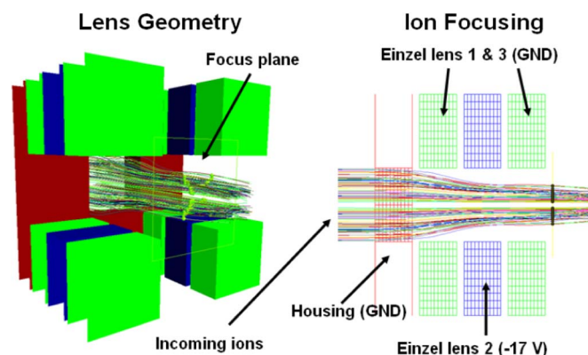
Fig. 4. Simulation of an Einzel lens with three sets of the unconventional lens elements in series.
