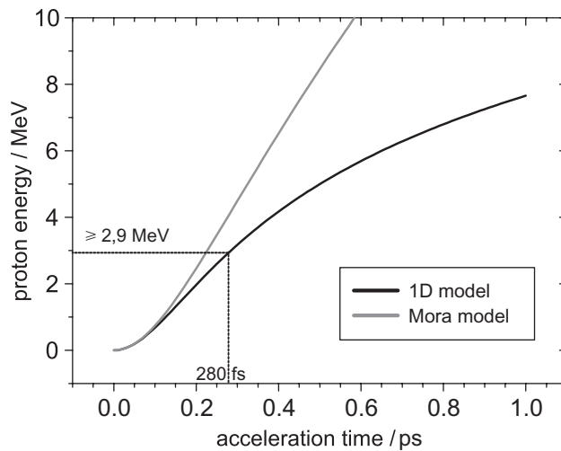
Figure 3. Maximum proton energy versus acceleration time.
