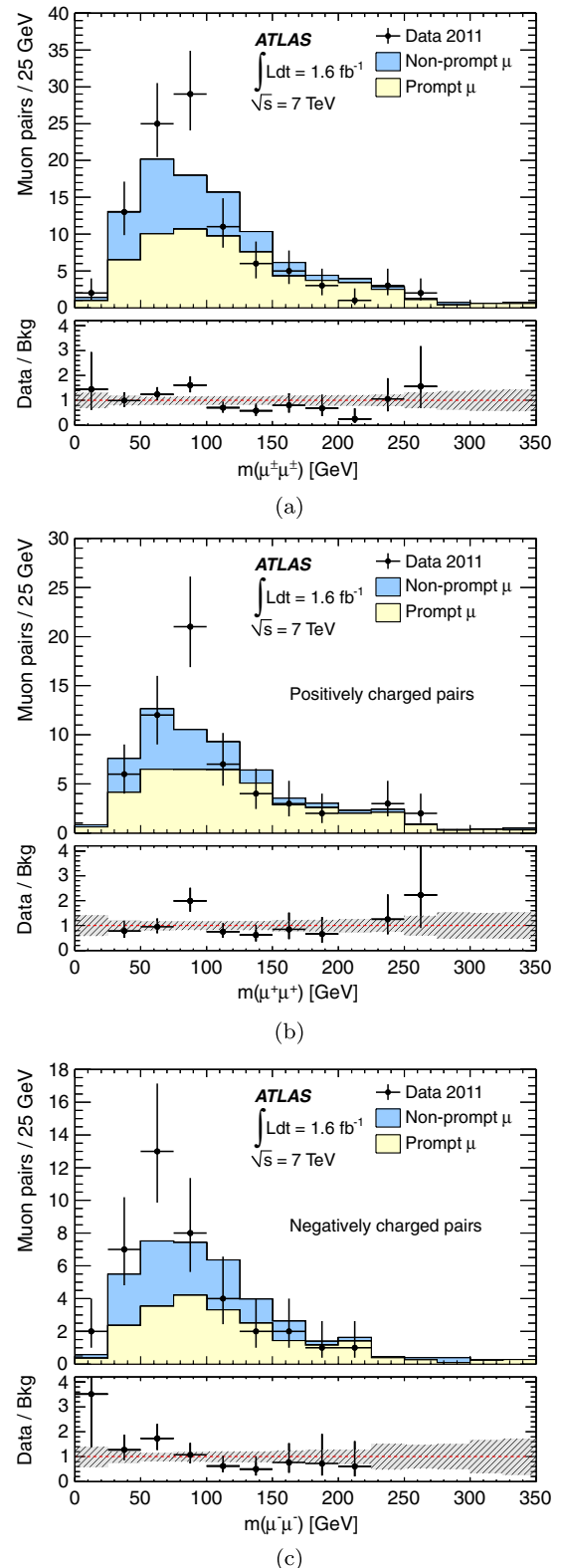
FIG. 1 (color online). Distribution of the dimuon invariant mass for (a) \mu^\pm\mu^\pm pairs, (b) \mu^+\mu^+ pairs, and (c) \mu^-\mu^- pairs. The data are compared to the stacked background estimates. The ratio between the data and the predicted background is also shown, where the shaded region is the total systematic uncertainty on the background prediction.
