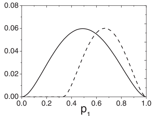
FIG. 4. The quantum discord (solid line) and entanglement (dashed line) of the state given in Eq. (9), with \rho_{\text{ent}} = |\Phi^+\rangle\langle\Phi^+| .
