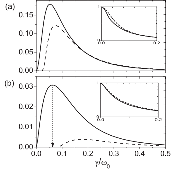
FIG. 1. Steady-state quantum discord (solid lines) and entanglement (dashed lines) between the qubits plotted against dissipation rate \gamma for N = 2 , J = 0.2\omega_0 , \Omega = 0.1\omega_0 , and \bar{n} = 0 . Both quantum correlations exhibit resonance behaviors. Insets are the quantum discord (solid lines) and the entanglement (dashed lines) between qubit 1 and the environment, according to Eq. (8). (a) At \Gamma = 0 . (b) At \Gamma = 0.15\omega_0 , the discord resonance occurs when the entanglement is strictly zero, as pointed by the dotted arrow.
