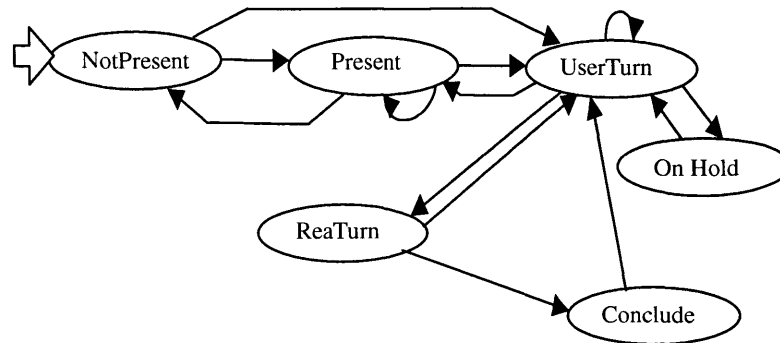
Figure 5.2: Conversational States in REA
