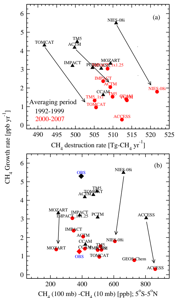
Fig. 11. Relationships of global loss rates for different models ( \text{CH}_4\text{-EXTRA} ) with their simulated growth rates at surface sites ( a ), and the modeled vertical gradients in the lower stratosphere (100–10 mb layer; b ) with growth rate. ACTM.OH and GEOS-Chem.DOH are excluded from this analysis as those models used different OH fields.
