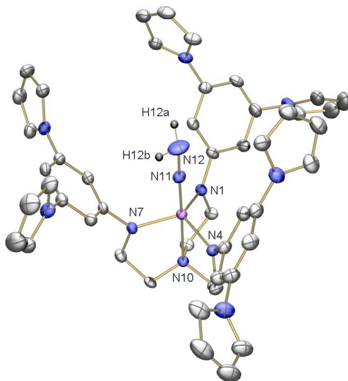
Figure 5. Thermal ellipsoid drawing of \{[\text{DPPN}_3\text{N}]\text{LMoN}_2\text{H}_2\}[\text{BAr}_4^f]\cdot[\text{C}_6\text{H}_6]\cdot 2.5[\text{C}_5\text{H}_{12}] with ellipsoids at 50% probability. Isopropyl groups, [\text{BAr}_4^f]^- anions, hydrogen atoms (except for H12a and H12b), and solvent molecules are omitted for clarity.
