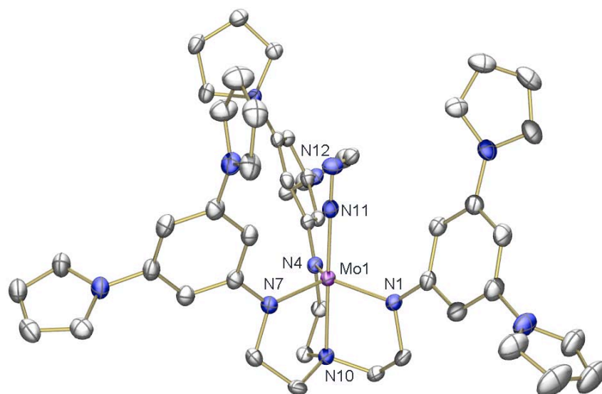
Figure 3. Thermal ellipsoid drawing of [\text{Bu}_4\text{N}][\{\text{DPPN}_3\text{N}\}\text{MoN}_2] \cdot 5[\text{C}_6\text{H}_6] with ellipsoids at 50% probability. Isopropyl groups, [\text{Bu}_4\text{N}]^+ , hydrogen atoms, and solvent molecules are omitted for clarity.
