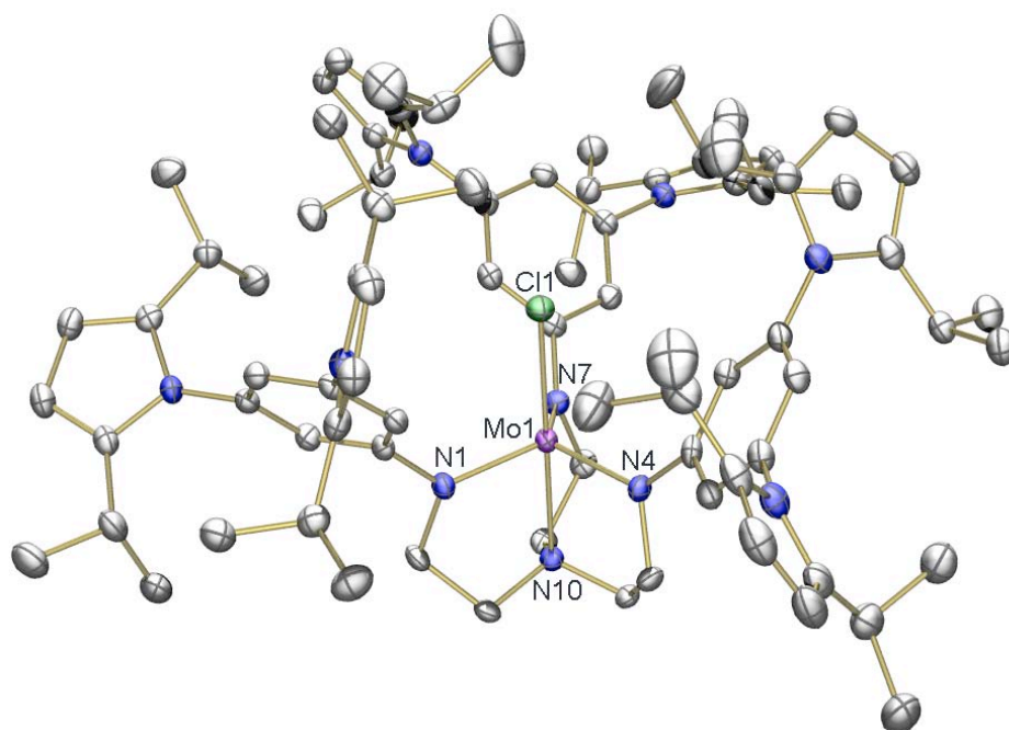
Figure 2. Thermal ellipsoid drawing of [DPPN 3 N]MoCl 2 ·2[(C 2 H 5 ) 2 O] with ellipsoids at 50% probability. Hydrogen atoms and solvent molecules are omitted for clarity.
