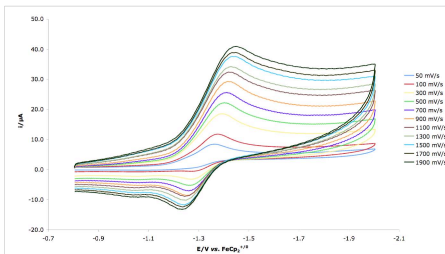
Figure 8. Cyclic voltammogram of {[DPPN 3 N]MoNH 3 }[BAr 4 f ] in PhF (0.1 M [Bu 4 N][BAr 4 f ]) at different scan rates. (Measured under an Argon atmosphere.)
