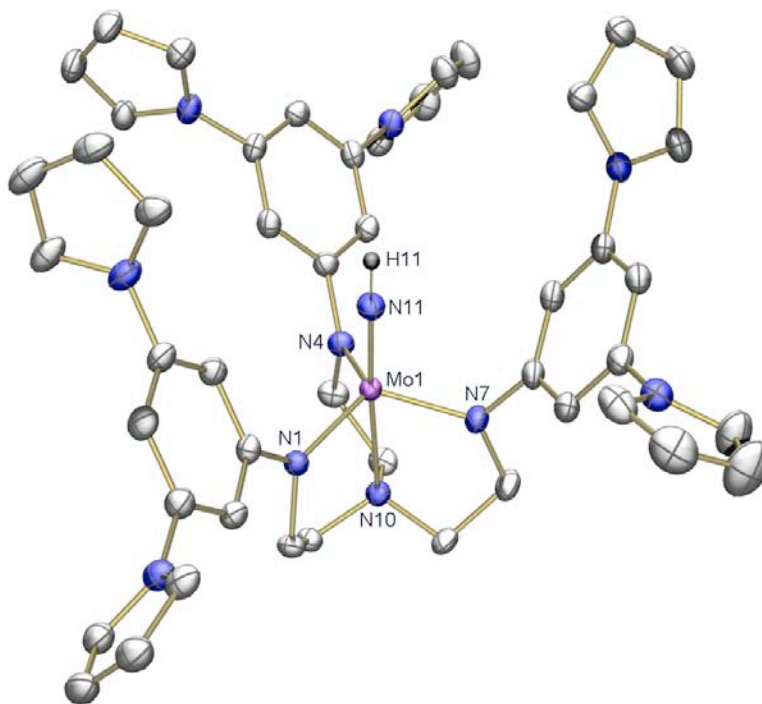
Figure 7. Thermal ellipsoid drawing of the first crystallographically independent molecule of \{[\text{DPPN}_3\text{N}]\text{Mo}\equiv\text{NH}\}^+ with ellipsoids at 50% probability. Isopropyl groups, [\text{BAr}^f_4]^- anions, hydrogen atoms (except for H11), and solvent molecules are omitted for clarity.
