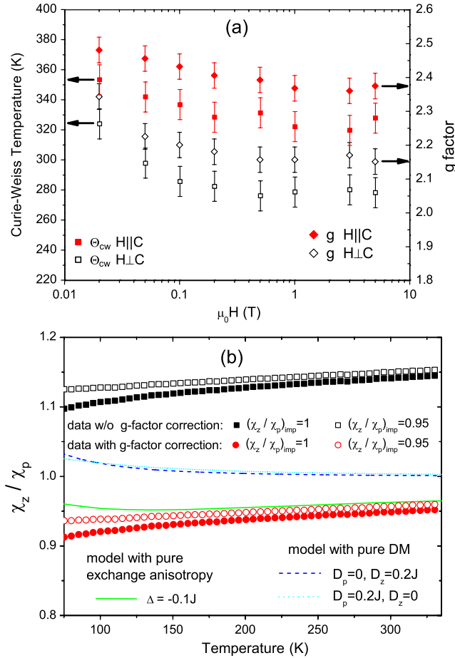
FIG. 3 (color online). (a) Curie-Weiss temperatures and g factors calculated from fits of the magnetic susceptibilities between T = 150 and 330 K, as described in the text. The proper vertical scale for each data set is indicated by the arrow. (b) The susceptibility anisotropy ratio of the intrinsic kagome spins after subtracting the impurity contribution, with and without a correction for the g -factor anisotropy, as described in the text. In the model for subtracting the impurity contribution, temperature independent anisotropy ratios (\chi_z/\chi_p)_{imp} were assumed. The three curves represent exact diagonalization calculations [11] for the anisotropy ratio considering the effects of an easy-axis exchange anisotropy and a DM interaction separately.
