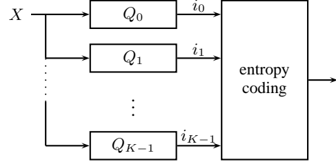
Fig. 1. Use of K dithered uniform scalar quantizers in parallel. Quantizer Q_k has thresholds \{(j + a_k)\Delta\}_{j \in \mathbb{Z}} , with a_k its offset .
