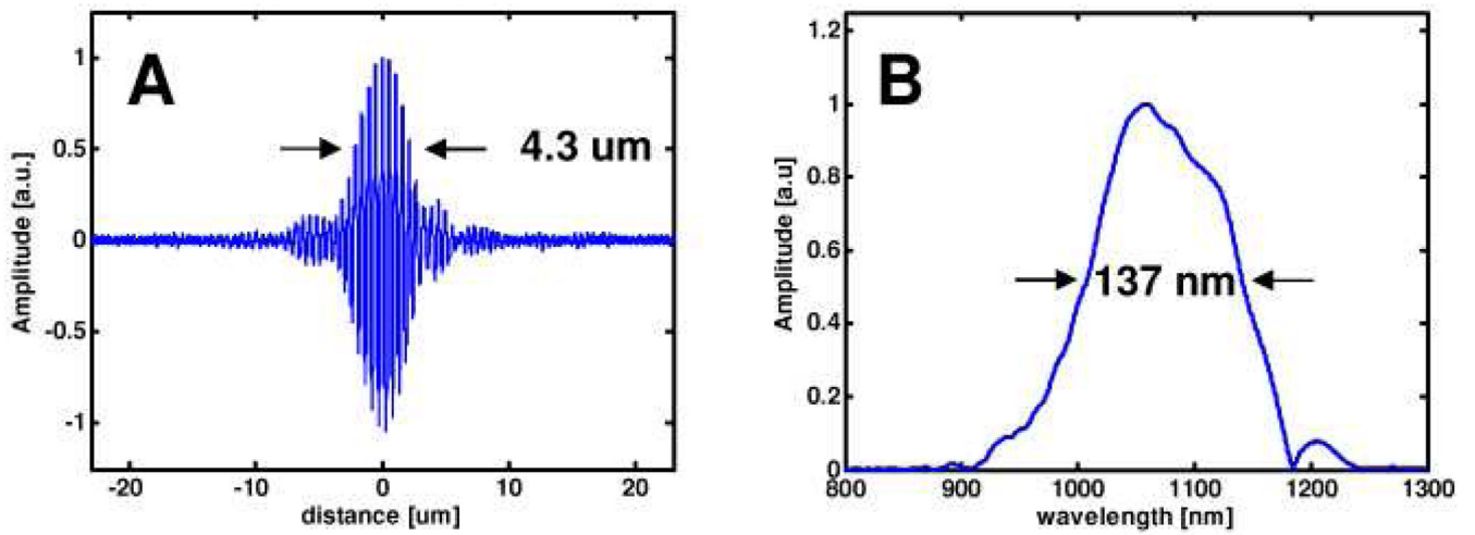
Fig. 3. Dispersion-balanced axial coherence point spread function achieved with polarization management. The axial resolution (a) measured 4.3\ \mu\text{m} in air, corresponding to 3.1\ \mu\text{m} in tissue. The Fourier transform of the point spread function (b), measures \sim 137\ \text{nm} in spectral full-width at half maximum
