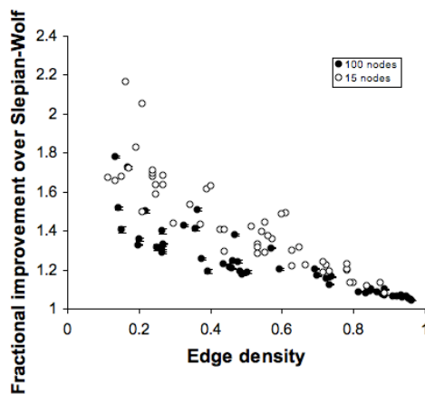
Fig. 4. Graph of the performance of the GA relative to the Slepian-Wolf bound for fifty 15-node and fifty 100-node graphs of varying edge densities, with 5 trials run on each graph. The y -axis shows the averaged values of \frac{H_G^\lambda(C, X|Y)}{H(X|Y)} for each graph, the fractional improvement over the Slepian-Wolf bound given by the best coloring C discovered by the GA. Error bars representing the standard deviation are shown for the 100-node graphs; in the 15-node case, the GA discovered identical (presumably optimal) values in all trials for all but two of the graphs.
