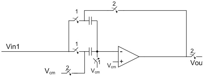
Figure 2. Amplification and Integration using the same switched-capacitor circuit
