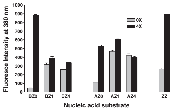
Figure 5. Comparison of fluorescence intensity at different 2-AP positions with and without Z \alpha . Fluorescence intensity of substrates containing no Z \alpha protein (0 \times , grey bars) was compared with that in the presence of a 4-fold excess of Z \alpha over nucleic-acid substrates (4 \times , solid bars). Intensity numbers were taken from fluorescence intensities at 380 nm for each nucleic-acid substrate. All measurements were repeated three times and results were averaged.
