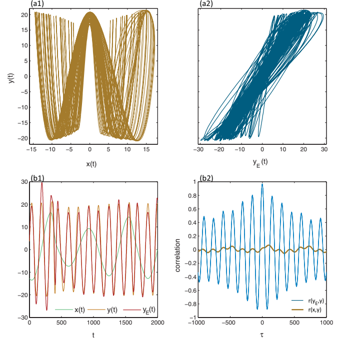
FIG. 4. (Color online) Identification of interaction between unidirectionally coupled Rössler systems in 4 : 1 phase synchronization [Eq. (15)]. (a1) Nonlinear synchronization manifold projected onto first coordinates x_1, x_2 of the two systems (brown). (a2) Linearized synchronization manifold after application of a fourth-order Volterra series operator (blue). (b1) Time domain plots of original signals x(t) [green (light gray)] and y(t) [orange (gray)] compared to the fourth-order model prediction y_E(t) [red (dark gray)]. (b2) Delay-shifted (by \tau ) correlation plots of original signals r(x,y) (brown, thick) and model performance r(y_E,y) (blue, thin). Bootstrapped confidence intervals are shown as dashed lines in light blue.
