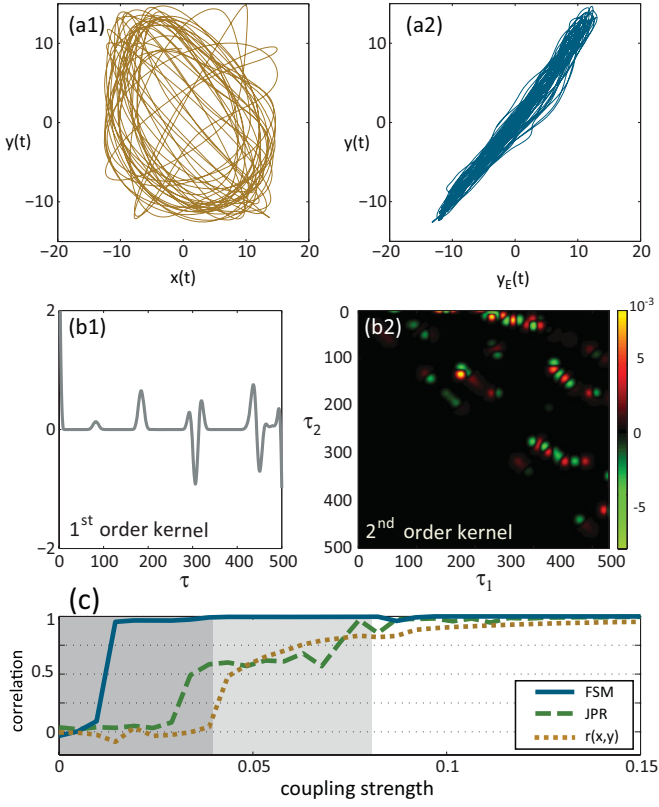
FIG. 3. (Color online) Identification of nonlinear interaction between coupled Rössler systems. (a1) Nonlinear synchronization manifold between original sampled data x and y (the systems' first coordinates) at onset of phase synchronization ( \mu = 0.034 ) with correlation r(x,y) \approx 0 . (a2) Linearized manifold between y_E and y , where y_E(t) = F[x](t) is the output of a second-order Volterra model, yielding r(y_E,y) = 0.97 . (b1) First-order kernel corresponding to (a2). (b2) Second-order kernel corresponding to (a2). (c) As \mu increases, the system transitions from unsynchronized, via phase ( \mu > 0.04 ) to generalized chaotic synchronization ( \mu > 0.08 ). Performance of the method (FSM, r(y_E,y) \in [-1,1] ) for various coupling strengths \mu is compared to correlation of the raw data r(x,y) , as well as the JPR \in [0,1] .
