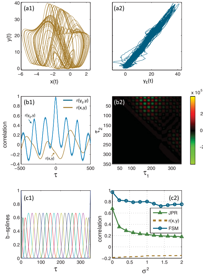
FIG. 1. (Color online) Identification of nonlinear interaction in a coupled Rössler-Lorenz system. (a1) Nonlinear synchronization manifold between original sampled data x and y (the systems' third coordinates) in generalized synchronization with correlation r(x, y) = -0.168 . (a2) Linearized manifold between y_E and y , where y_E(t) = F[x](t) is the output of a second-order Volterra model, yielding r(y_E, y) = 0.98 . (b1) Delay-shifted (by \tau ) correlation coefficients. (b2) Second-order kernel corresponding to (a2). (c1) Set of cubic b splines corresponding to (b2), used in Eq. (3). (c2) Performance of the method (FSM, r(y_E, y) \in [-1, 1] ) for Rössler-Lorenz system with additive white noise over increasing variance \sigma^2 , compared against correlation r(x, y) , as well as the JPR \in [0, 1] .
