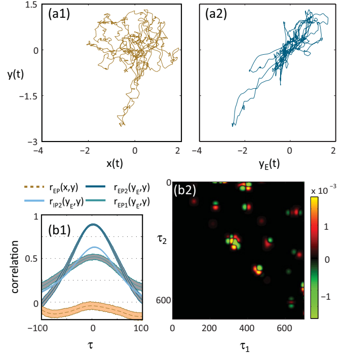
FIG. 5. (Color online) Two macaque V1 LFP recordings x and y recorded from electrodes with different retinotopy. (a) Interaction manifolds of the EPs. (a1) Nonlinear manifold between x and y . (a2) Linearized manifold corresponding to r_{EP2}(y_E, y) in (b1). (b1) Lagged correlation coefficient between EPs of x and y [ r_{EP}(x, y) ], and between a first-order [ r_{EP1}(y_E, y) ] and second-order [ r_{EP2}(y_E, y) ] model y_E = F[x] and predicted tetrode y . For the IPs correlations are shown between a second-order model y_E and y [ r_{IP2}(y_E, y) ]. Lighter colored areas show the bootstrapped confidence intervals of the respective models. (b2) Shows the second-order kernel.
