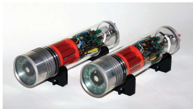
Fig. 1. Two AquaOptical II modems.
