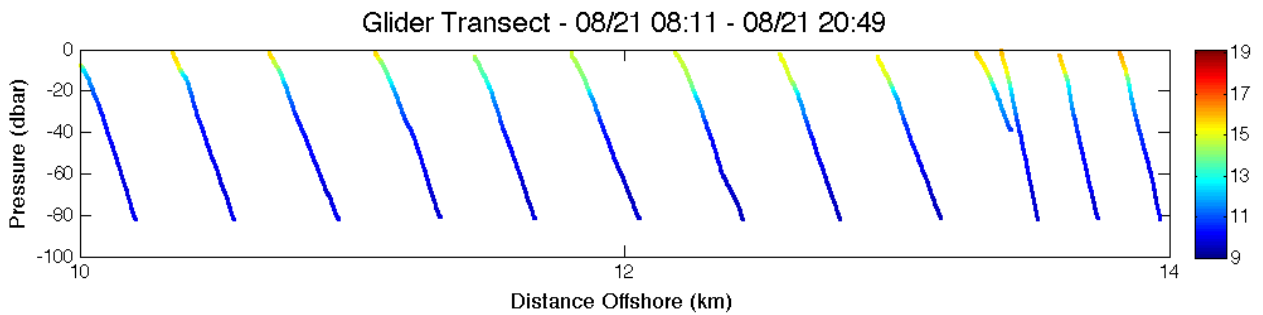
(b) Temperature data with 26° pitch angle.
