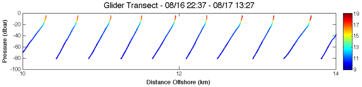
(a) Temperature data with 15° pitch angle.
