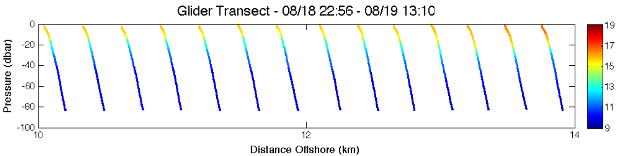
(c) Temperature data with 35° pitch angle.
