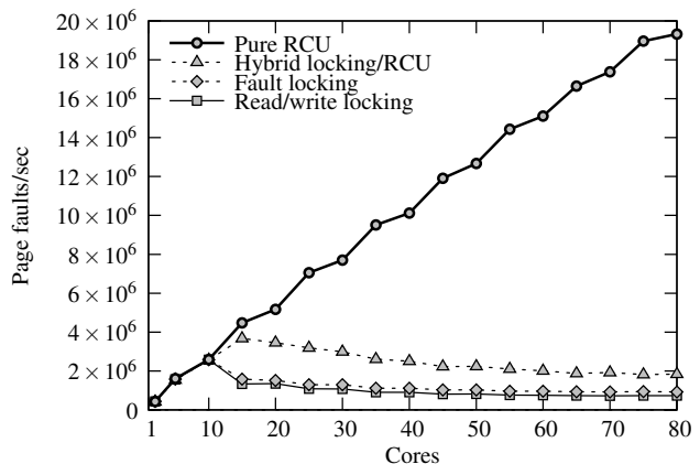
Figure 16. Microbenchmark throughput with no lock contention.
