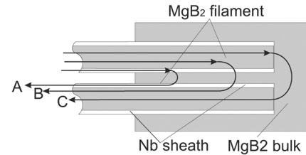
Fig. 7. Paths for superconducting current from one wire to the other via the splice.
