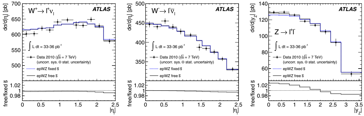
FIG. 1 (color online). Differential d\sigma/d|\eta_{\ell^+}| (left) and d\sigma/d|\eta_{\ell^-}| (middle) cross-section measurements for W \rightarrow \ell\nu and d\sigma/d|y_Z| cross-section measurement for d\sigma/d|y_Z| (right). The error bars represent the statistical and uncorrelated systematic uncertainties added in quadrature while the theoretical curves are adjusted to the correlated error shifts (see text). The NNLO fit results with free and fixed strangeness are also indicated, and their ratios are shown in the panels below the cross-section plots.
