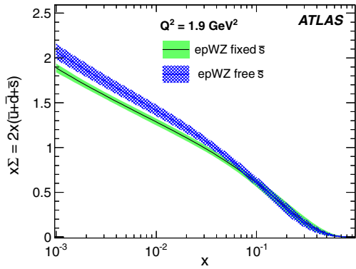
FIG. 3 (color online). Distribution of the light sea quarks, x\Sigma = 2x(\bar{u} + \bar{d} + \bar{s}) , in the NNLO analysis of HERA and ATLAS data with a fixed fraction of strangeness (lower green curve) and with a fitted fraction of about unity (upper blue curve). The bands represent the experimental uncertainties.
