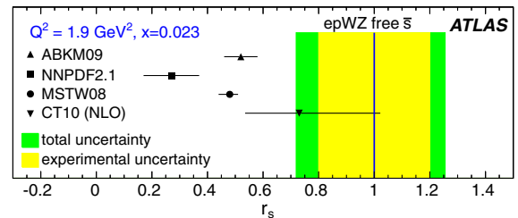
FIG. 2 (color online). Predictions for the ratio r_s = 0.5(s + \bar{s})/\bar{d} , at Q^2 = 1.9 \text{ GeV}^2 , x = 0.023 . Points: global fit results using the PDF uncertainties as quoted; bands: this analysis; inner band, experimental uncertainty; outer band, total uncertainty.
