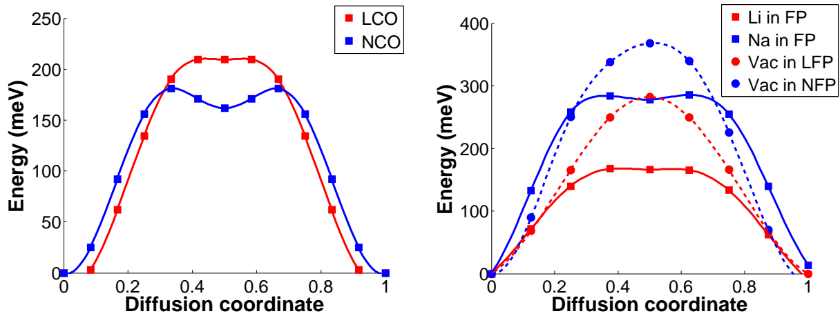
(a) Barrier for divacancy diffusion mechanism in layered \text{ACoO}_2 (b) Barriers for (i) alkali (A) diffusion in dealkaliated olivine \text{FePO}_4 (FP) and (ii) vacancy (V) diffusion in \text{AFePO}_4 (LFP and NFP)
