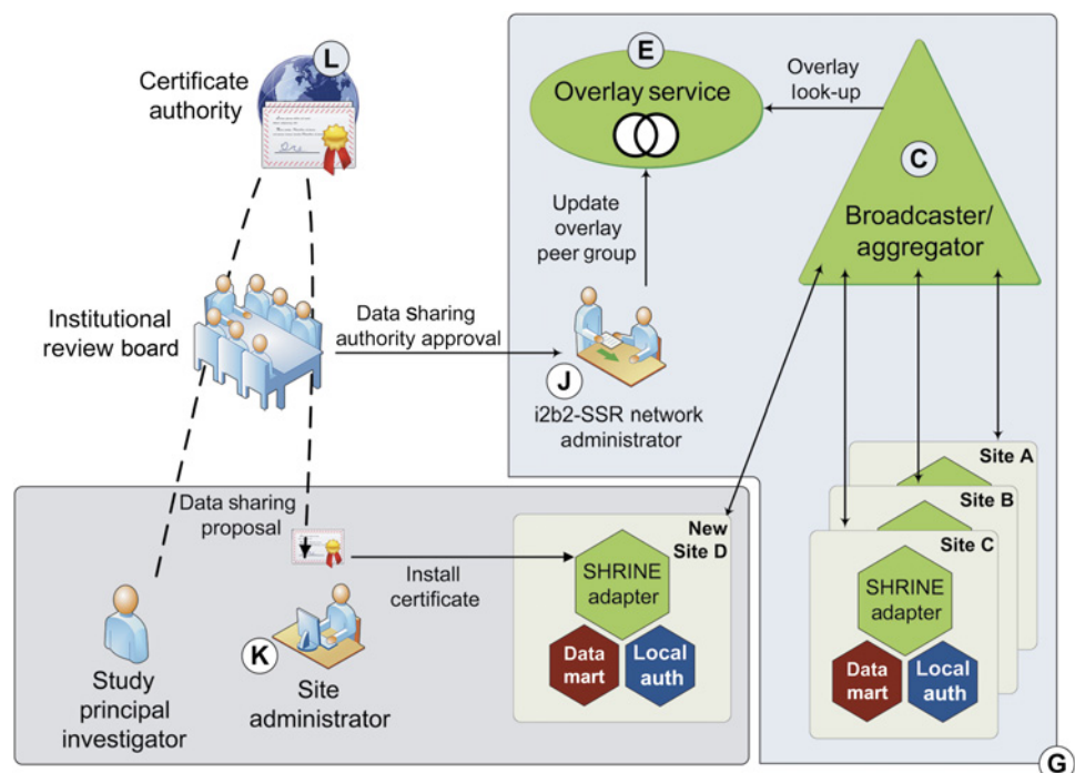
Figure 3 Self-scaling architecture—adding new sites (network nodes) and/or studies to an i2b2-SSR network. With appropriate approvals, a Site Administrator (K) configures the local SHRINE adapter to communicate with a particular registry Broadcaster/Aggregator endpoint (C) and installs a digital certificate distributed by a certificate authority (L) that is mutually trusted by the site and the i2b2-SSR Network Administrator (J).
