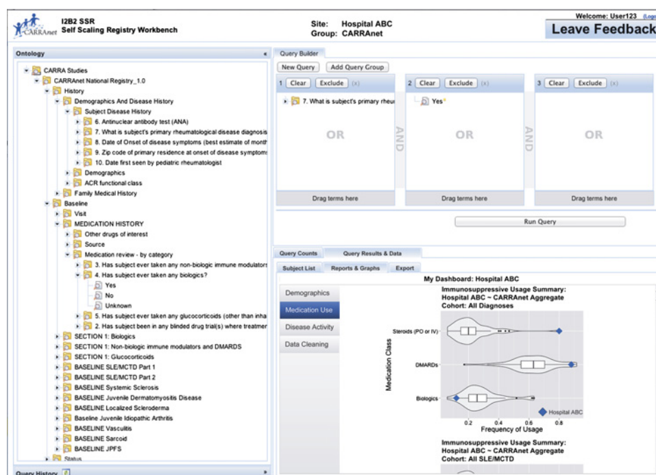
Figure 2 End user query interface. The Site Investigator dashboard view is shown, illustrating a sample visualization of summary statistics for site 'ABC' versus the entire CARRAnet registry.
