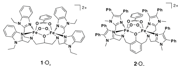
Chart 2 A proposed structure of [\text{Fe}_2(\mu\text{-O}_2)(N\text{-EtHPTB})(\text{PhCO}_2)]^{2+} ( 1\cdot\text{O}_2 , left). The benzoate ligand in 1\cdot\text{O}_2 may be coordinated in a terminal rather than bridging fashion. 37 The X-ray structure of [\text{Fe}_2(\mu\text{-O}_2)(\text{Ph-bimp})(\text{PhCO}_2)]^{2+} ( 2\cdot\text{O}_2 , right) has been determined. 39
