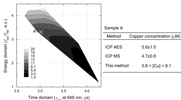
Figure 3. Contour map showing copper concentration as a function of phosphorescence intensity ratio ( I_{\text{ppp}}/I_{\text{btp}} ) and average phosphorescence lifetime ( \tau_{\text{avg}} ) of ZIr2. Also depicted is the quantitation of copper in sample A using the phosphorescence signals. At the right is a comparison of values determined by ICP AES, ICP MS, and the present method.
